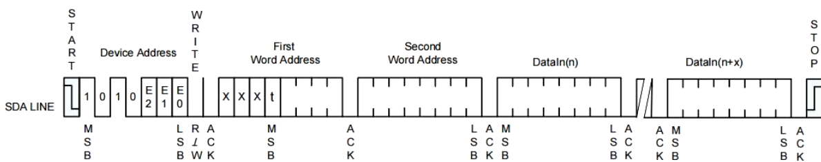
Figure 5-2 Page Write
