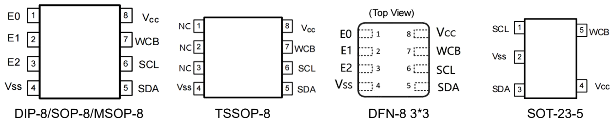
Figure 1-1 Pin Configuration
