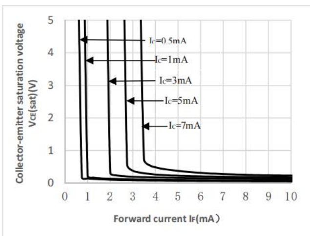
Fig.11 Collector-emitter Saturation Voltage vs. Forward Current
