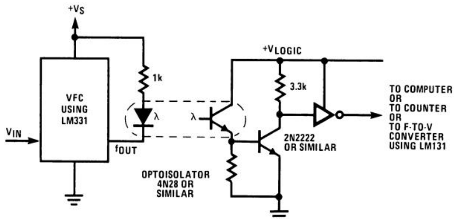
Figure 27. Voltage-to-Frequency Converter with Isolators
