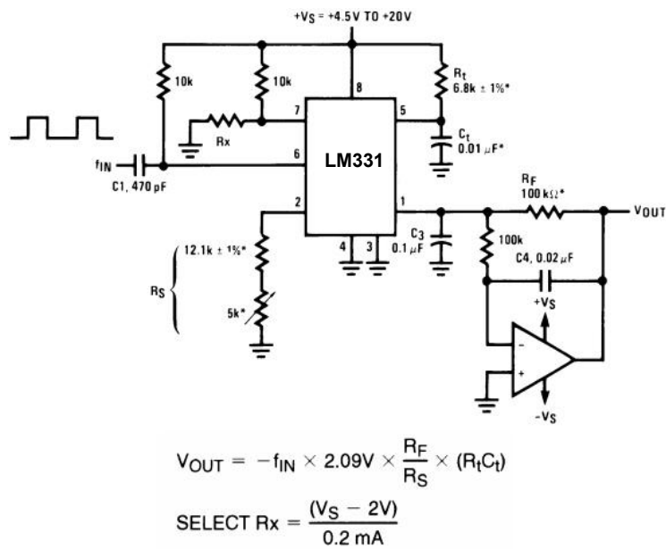
Figure 18. Simple Frequency-to-Voltage Converter, 10 kHz Full-Scale, \pm 0.06\% Non-Linearity
