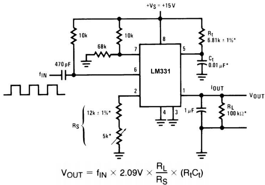
Figure 18. Simple Frequency-to-Voltage Converter, 10 kHz Full-Scale, \pm 0.06\% Non-Linearity
