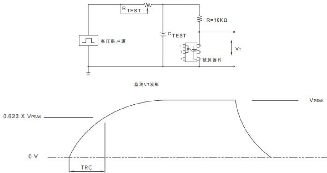
Fig.7 Static dv / dt test circuit and waveform
