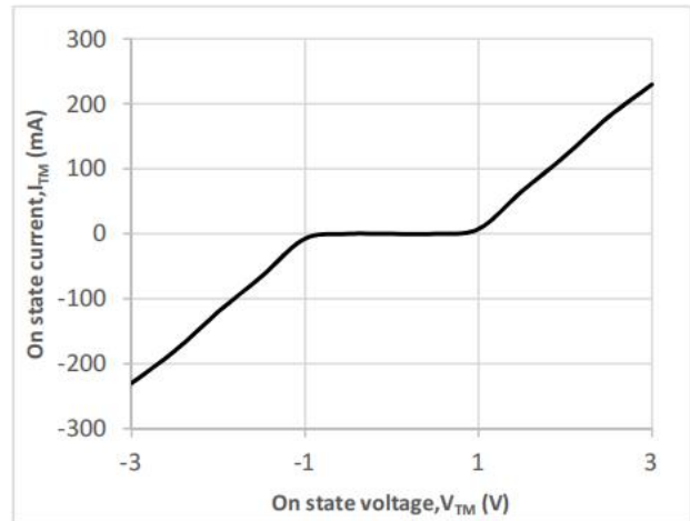
Fig.2 On-state characteristic
