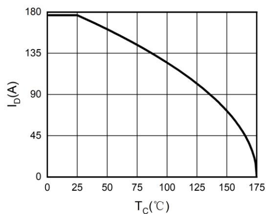
Figure 4. Drain Current
