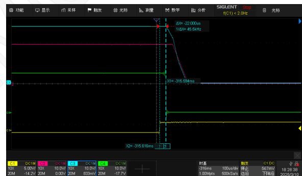
OVLO protection
