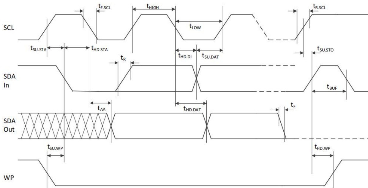
Figure 6-1 Bus Timing
