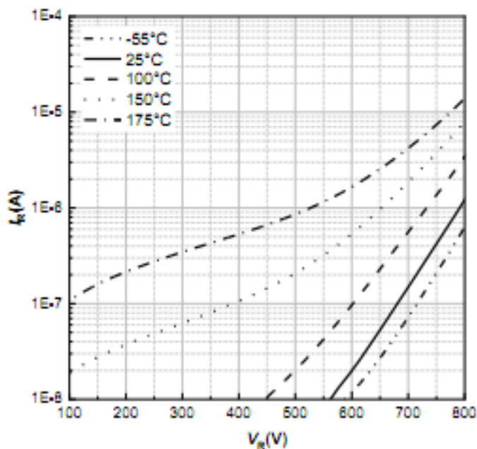
Figure 2. Typical reverse current as function of reverse voltage
