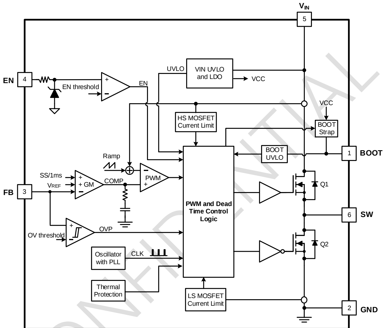
Figure 7. Block Diagram
