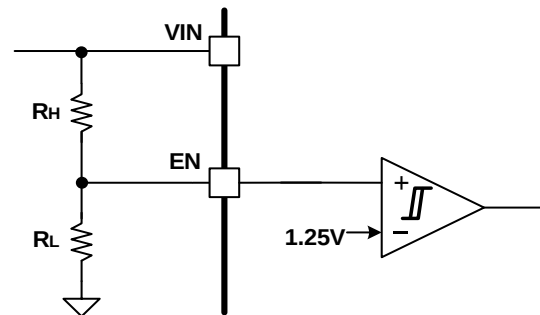
Figure 8. System UVLO by EN divider
