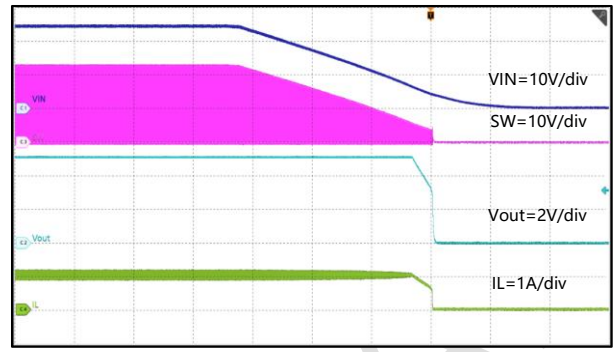
Figure 21. Shut-Down with VIN falling, I_{OUT}=1A
