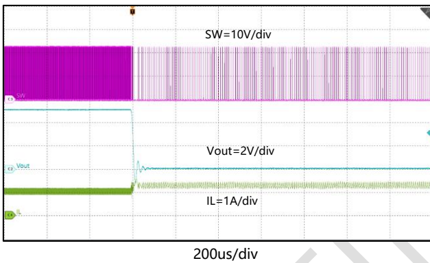
Figure 22. 1A Operation to HardShort, I_{OUT}=1A
