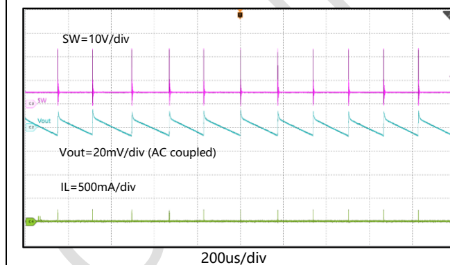
Figure 12. Output Voltage Ripple, I_{OUT} = 1\text{mA}
