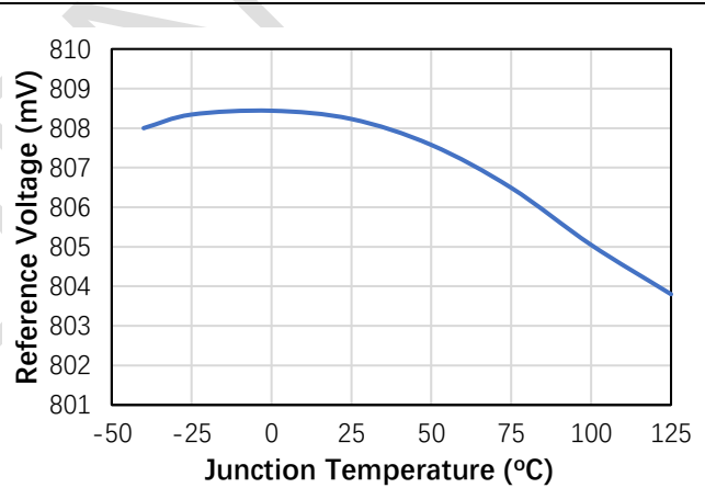
Figure 4. Reference Voltage vs. Junction Temperature
