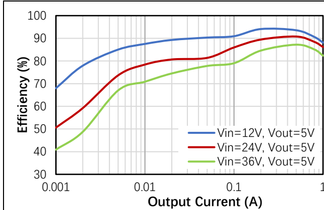
Figure 1. Efficiency Curve
