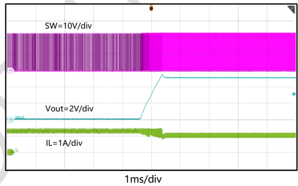
Figure 23. HardShort Recovery, I_{OUT}=1A
