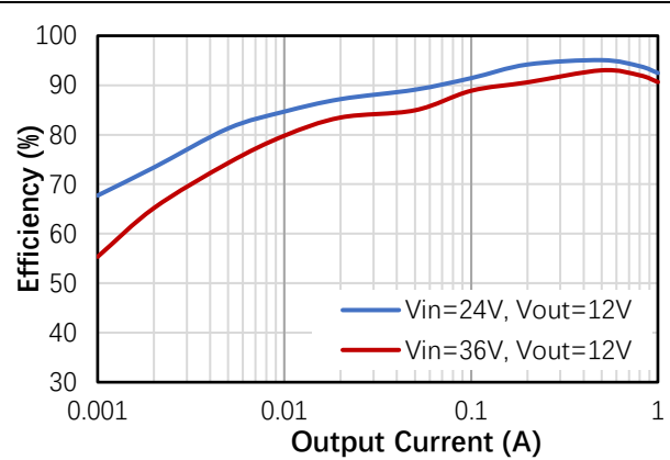
Figure 2. Efficiency Curve, L=22uH
