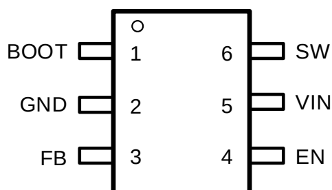
Top View: GBI1410 TSOT23-6L
