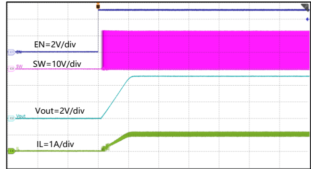
Figure 15. Start-Up with EN, I_{OUT}=1A
