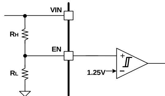
Figure 8. System UVLO by EN divider
