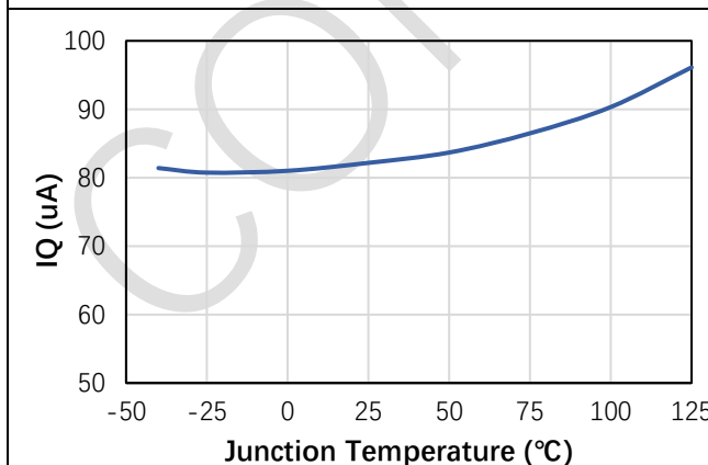
Figure 5. IQ vs Junction Temperature
