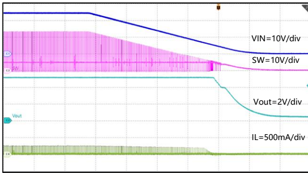
Figure 20. Shut-Down with VIN falling, I_{OUT}=1mA
