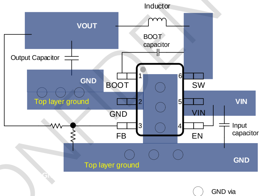
Figure 26. Layout Example
