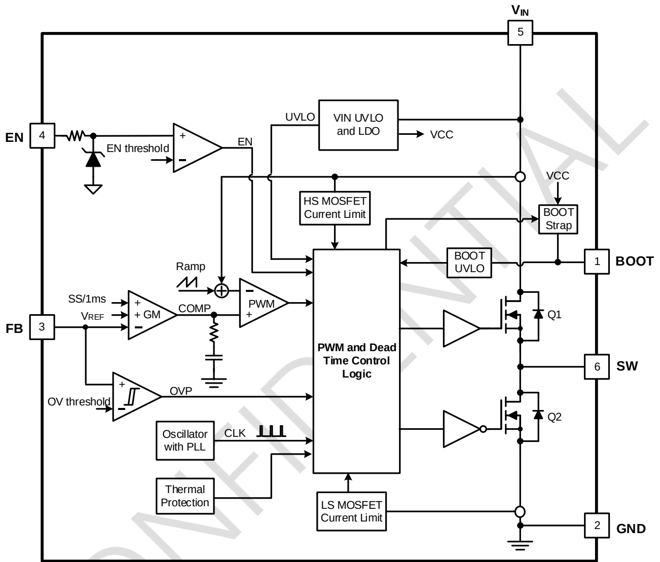
Figure 7. Block Diagram for GBI1410
