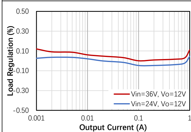
Figure 3. Load Regulation, L=22uH
