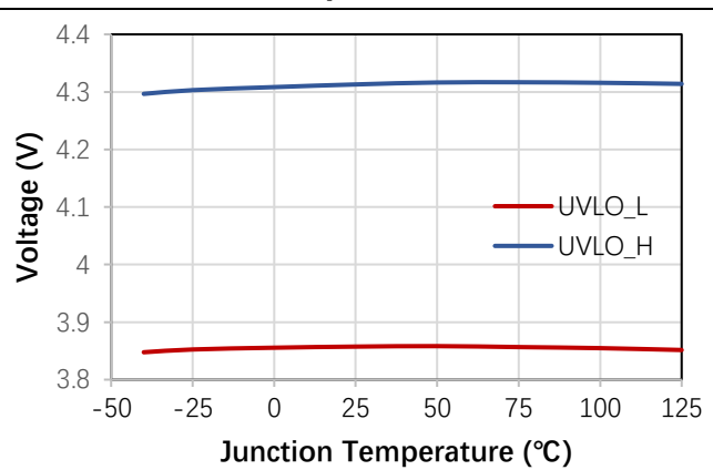
Figure 6. UVLO vs Junction Temperature
