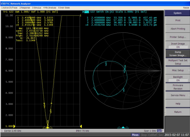
Fig.1 驻波比 VSWR
