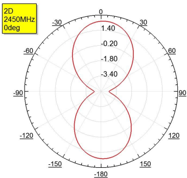
2D 增益模式 2D Gain Pattern (2450 MHz)
