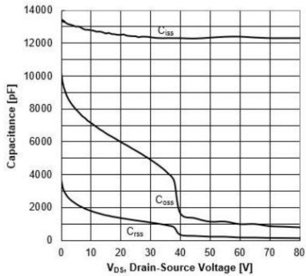
Figure 12. Capacitance Characteristics
