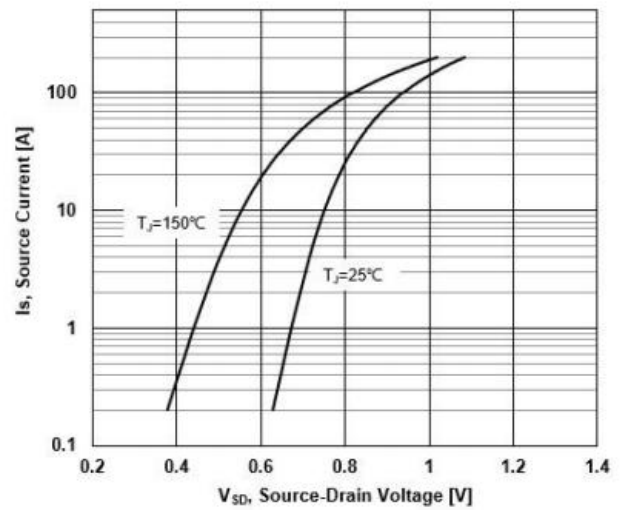
Figure 7. Source-Drain Diode Forward Characteristics
