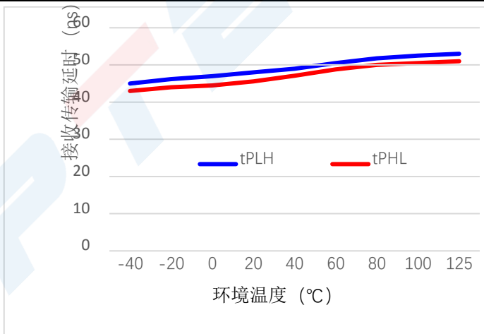
图 7.10-10 TDA51S485HC 接收传输延时, V_{CC} = 3.3\text{V} , V_{ISO} = 3.3\text{V} , R_L = 54\Omega
