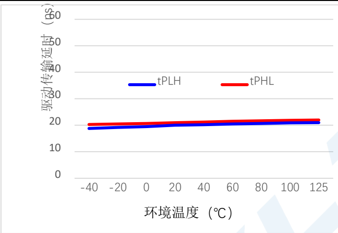
图 7.10-9 TDA51S485HC 驱动传输延时, V_{CC} = 3.3\text{V} , V_{ISO} = 3.3\text{V} , R_L = 54\Omega
