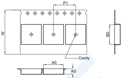
TAPE DIMENSIONS
