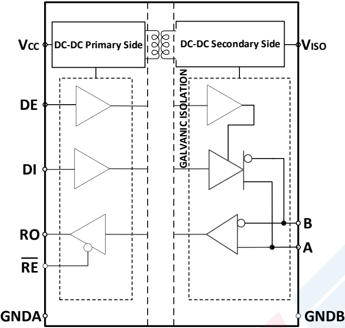
TDA51S485HC
