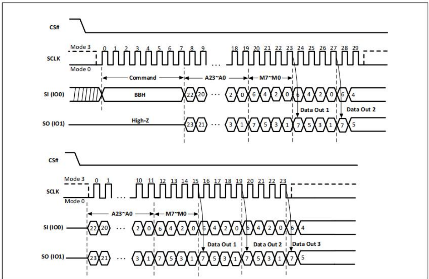
Figure-21. Dual I/O Fast Read with “Continuous Read Mode” Sequence Diagram (M5-4 = (1,0))
