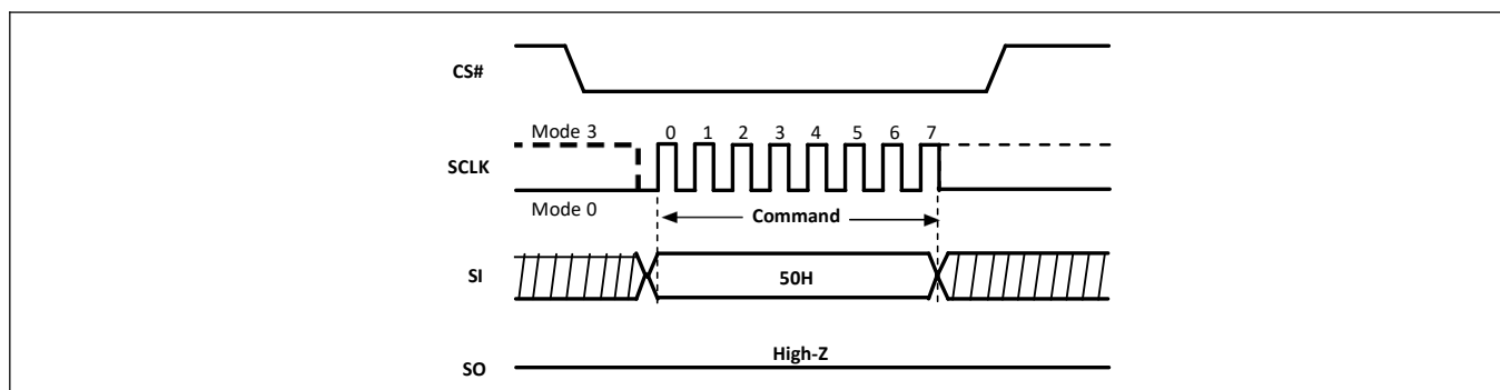
Figure-8. Write Enable for Volatile Status Register Sequence Diagram
