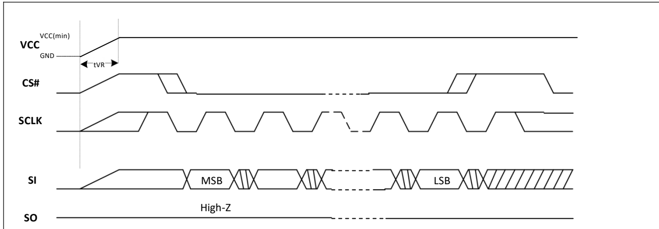
Figure-72. Power-On Timing Sequence Diagram
