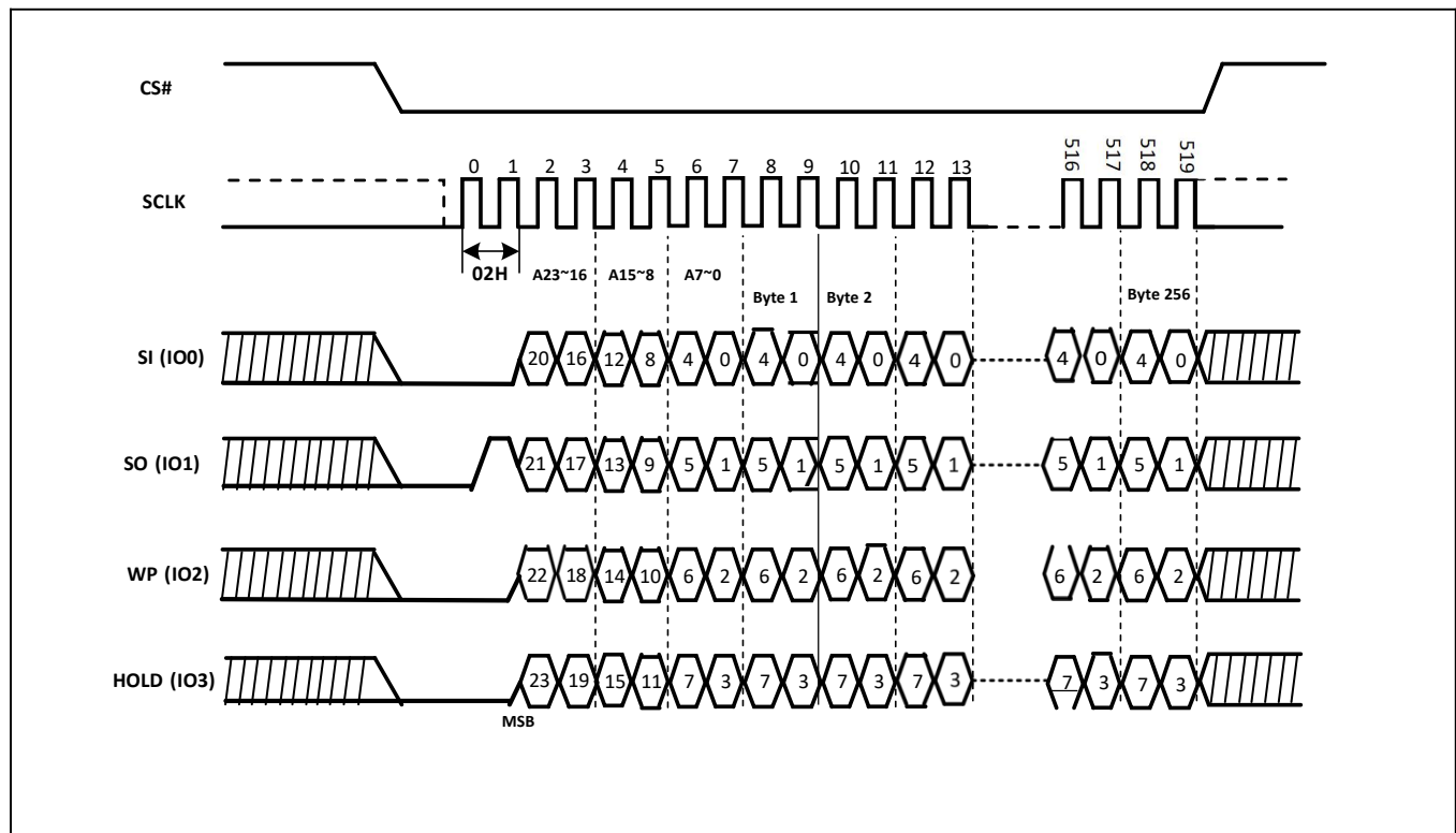
Figure-44. Page Program Sequence Diagram (QPI)
