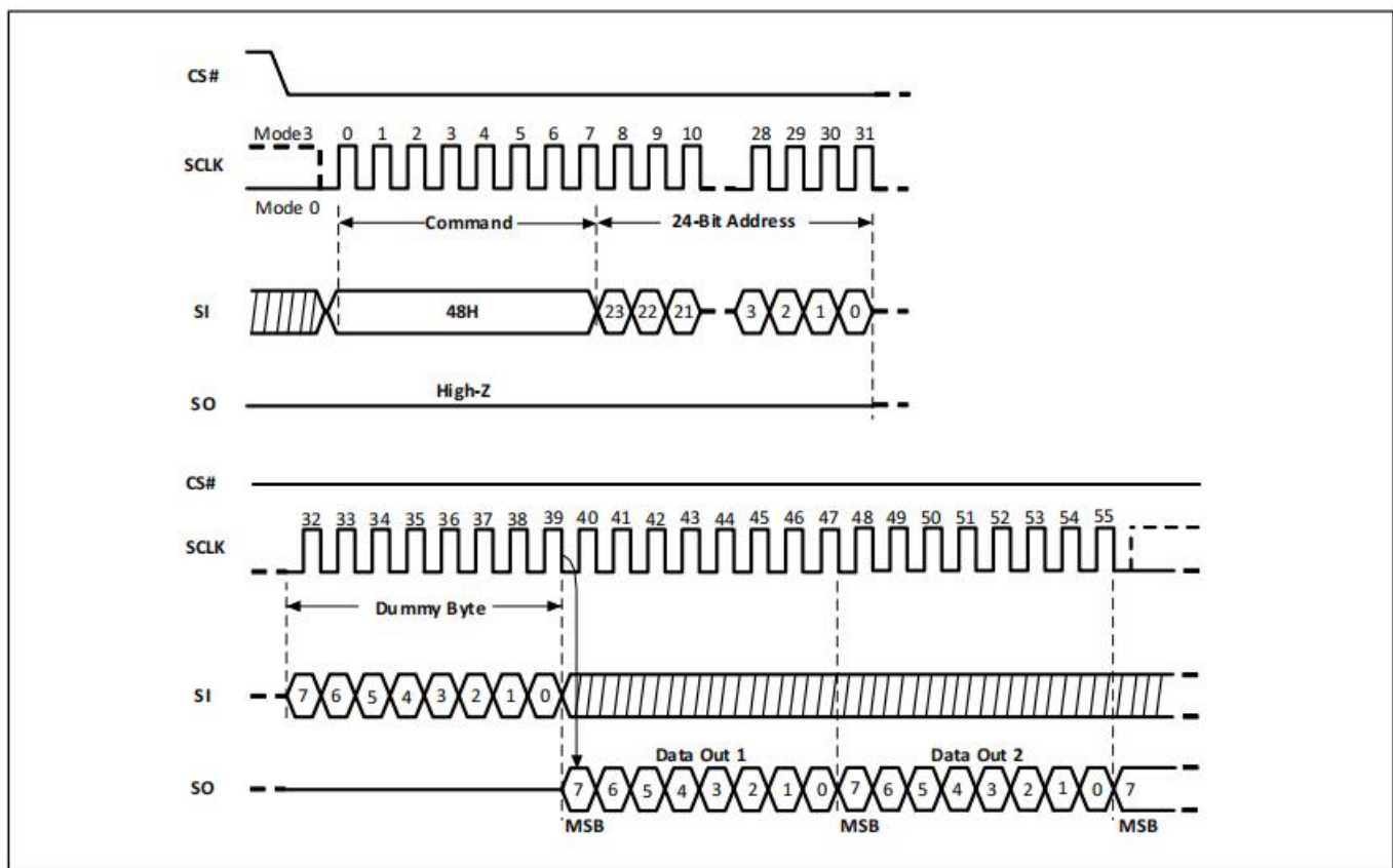
Figure-48. Read Security Register Sequence Diagram
