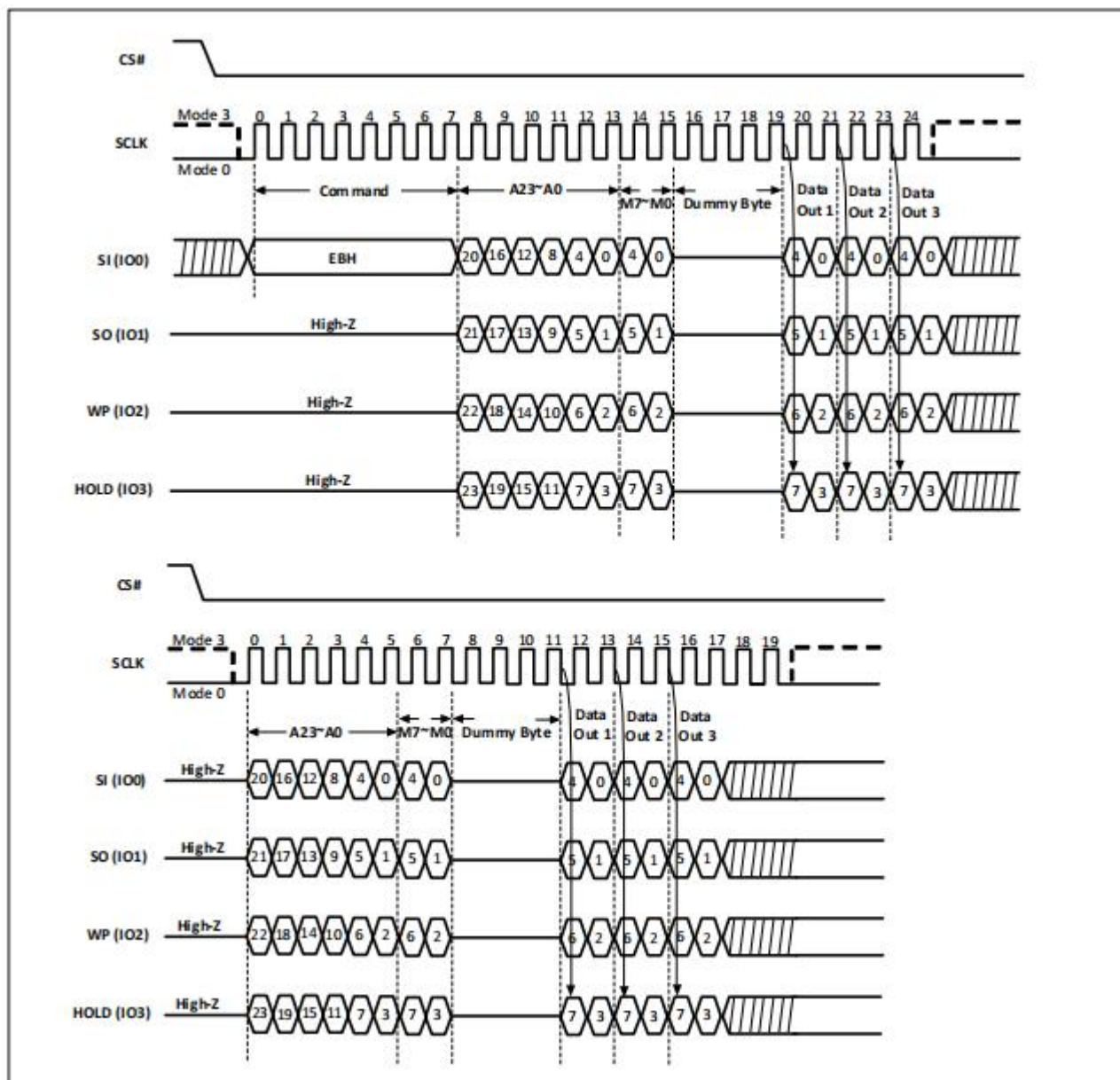
Figure-26. Quad I/O Fast Read with “Continuous Read Mode” Sequence Diagram (M5-4 = (1,0))
