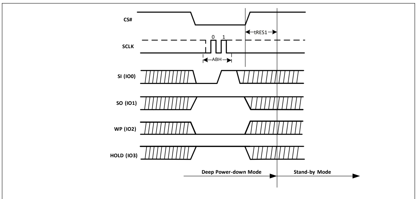
Figure-52. Release from Deep Power-Down (RDP) Sequence Diagram (QPI)
