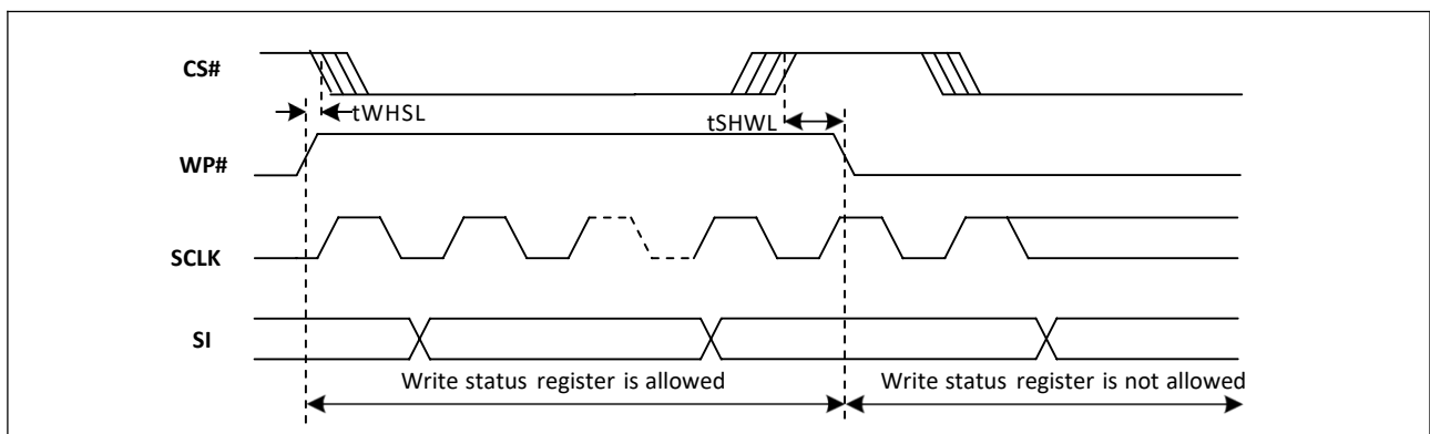
Figure-82. WP Timing
