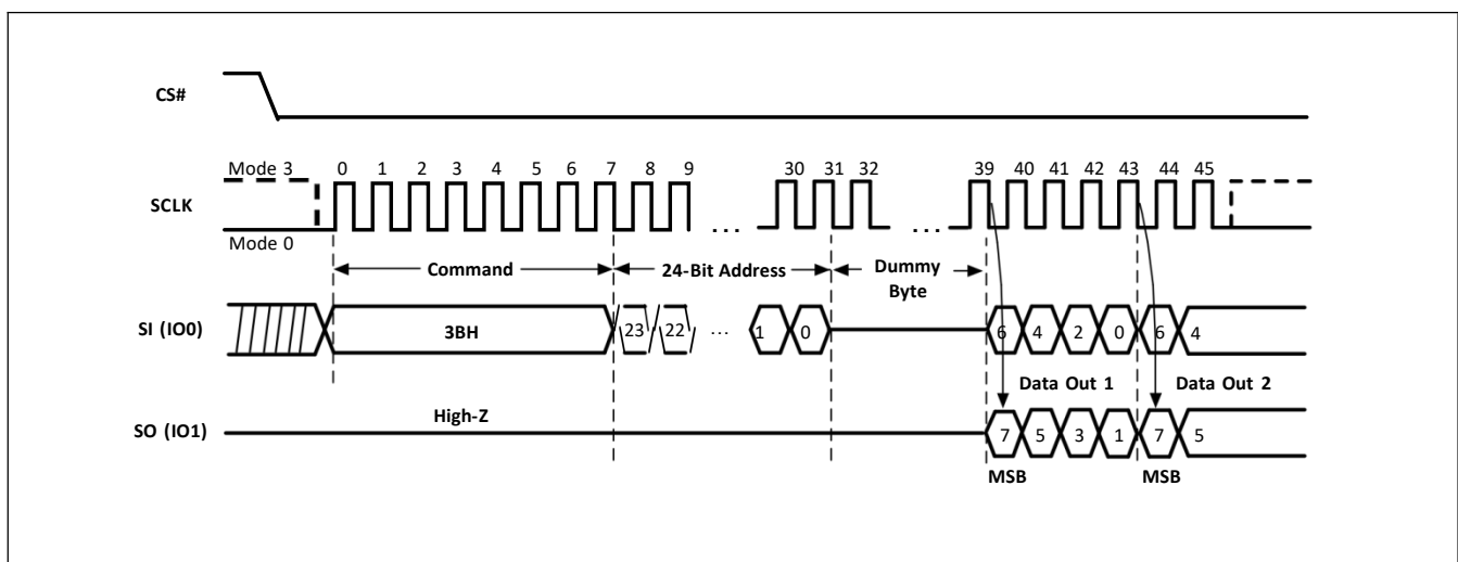
Figure-19. Dual Output Fast Read Sequence Diagram
