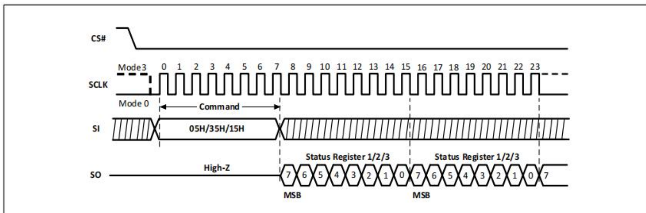
Figure-10. Read Status Register Sequence Diagram
