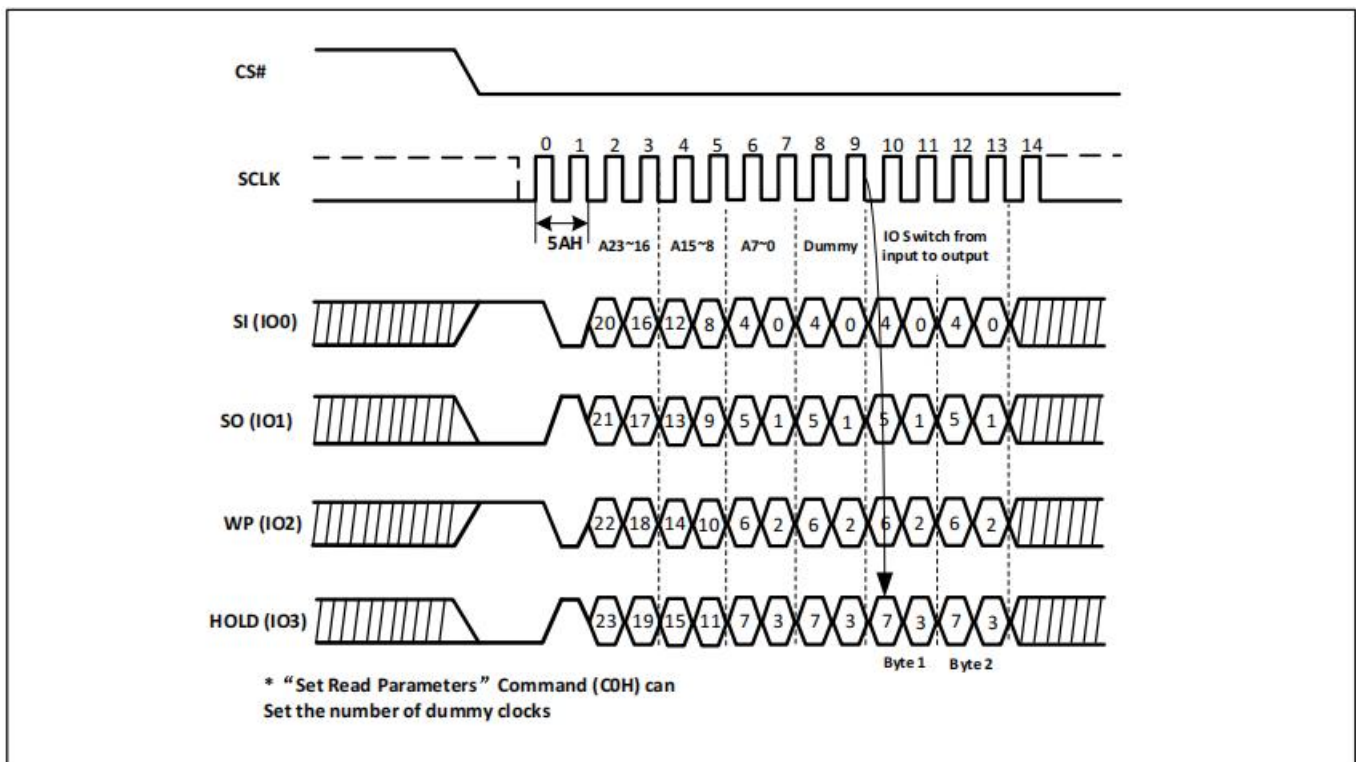
Figure-65. Read Serial Flash Discoverable Parameter Sequence Diagram (QPI)
