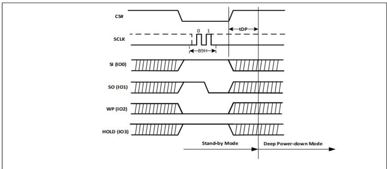
Figure-50. Deep Power-Down Sequence Diagram (QPI)
