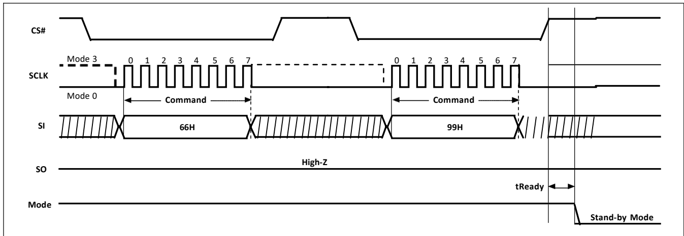
Figure-69. Reset Enable and Reset Sequence Diagram
