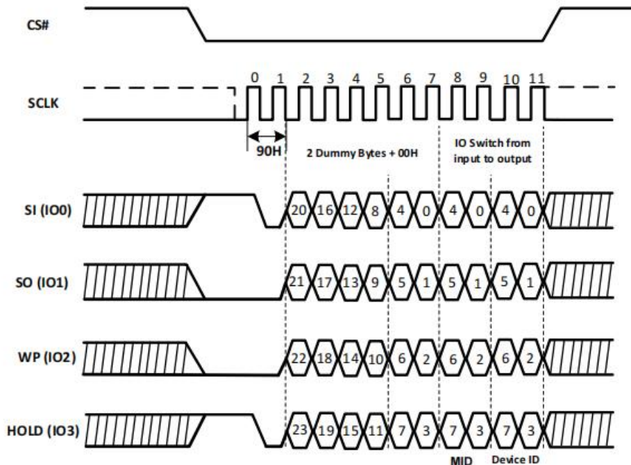
Figure-56. Read Electronic Manufacturer ID & Device ID Sequence Diagram (QPI)
