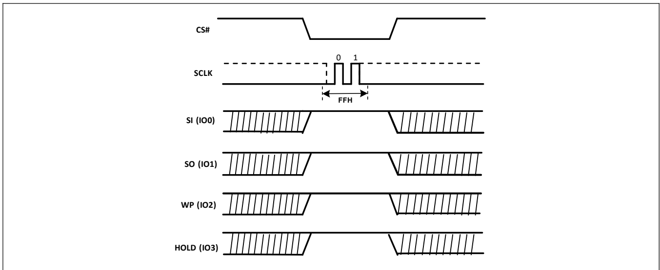
Figure-68. Disable QPI (QPI)
