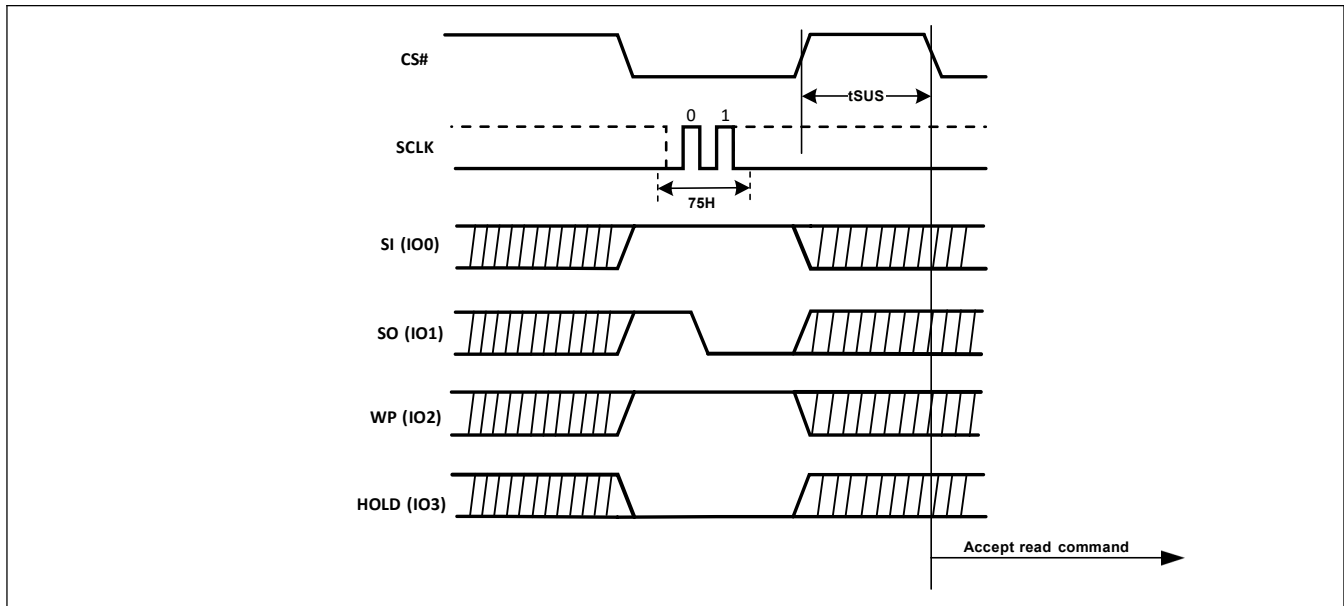
Figure-60. Program/Erase Suspend Sequence Diagram (QPI)
