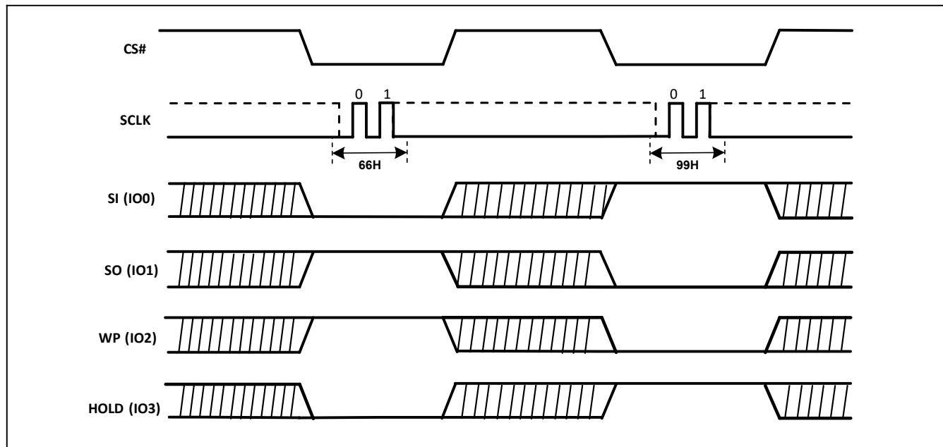
Figure-70. Reset Enable and Reset Sequence Diagram (QPI)
