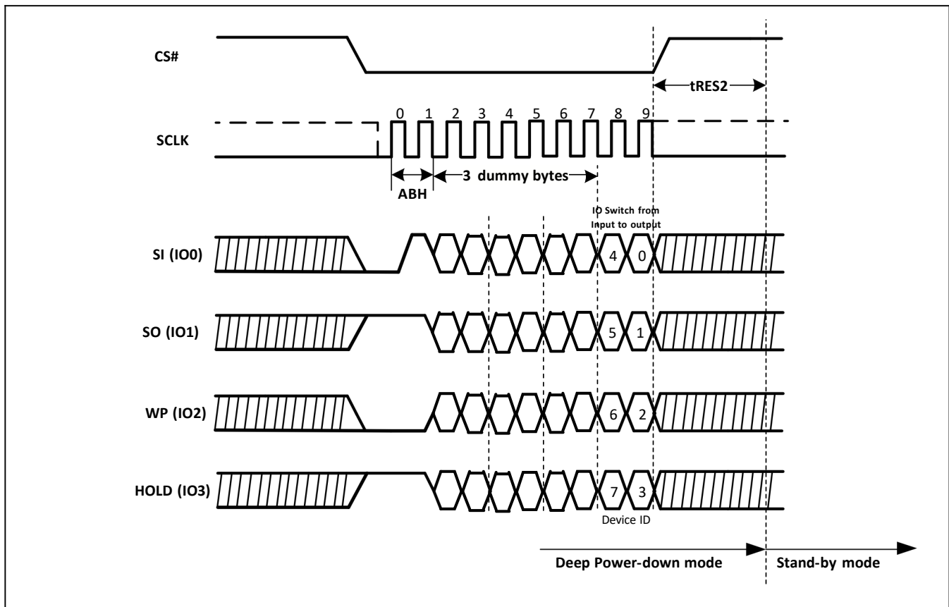
Figure-54. Read Electronic Signature (RES) Sequence Diagram (QPI)
