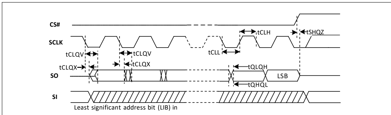
Figure-80. Output Timing (DTR mode)
