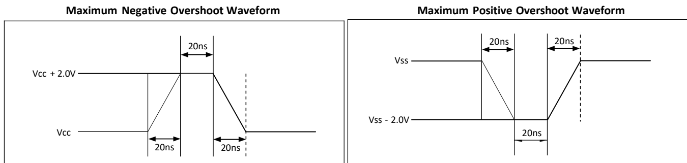
Figure-74. Maximum Negative/positive Overshoot Diagram
