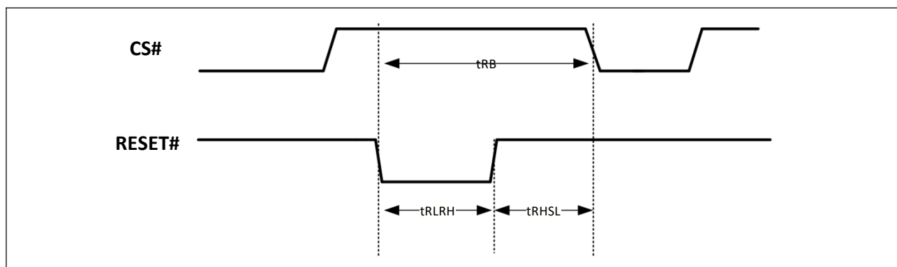
Figure-84. RESET Timing
