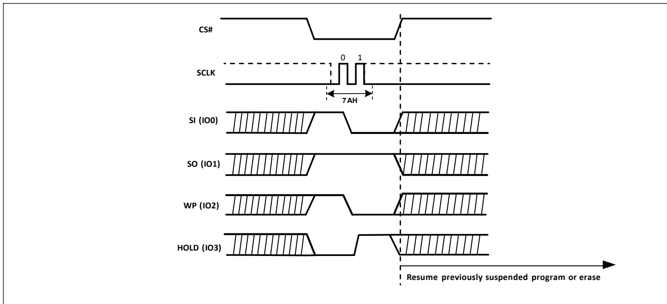
Figure-62. Program Resume and Erase Resume Sequence Diagram (QPI)
