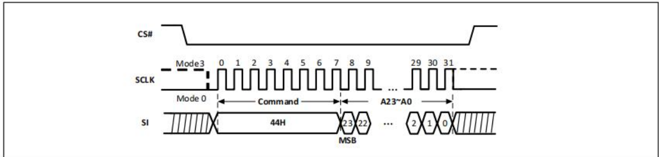
Figure-46. Erase Security Register Sequence Diagram
