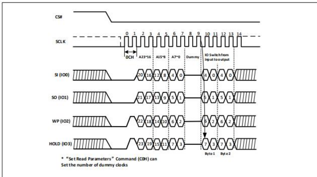
Figure-32. Burst Read with Wrap Sequence ( QPI )
