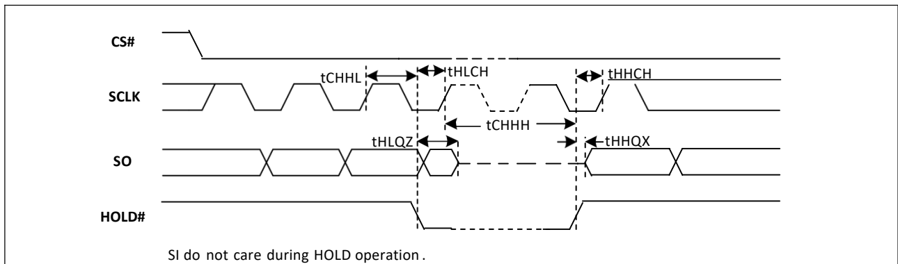
Figure-81. Hold Timing
