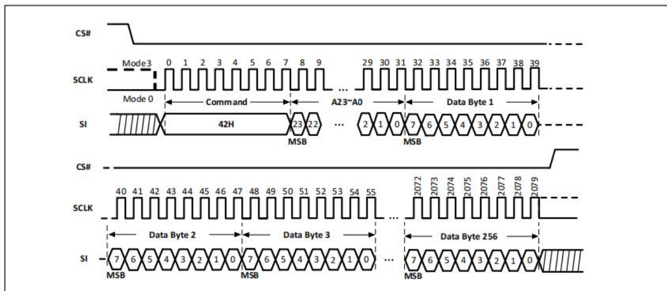
Figure-47. Program Security Register Sequence Diagram
