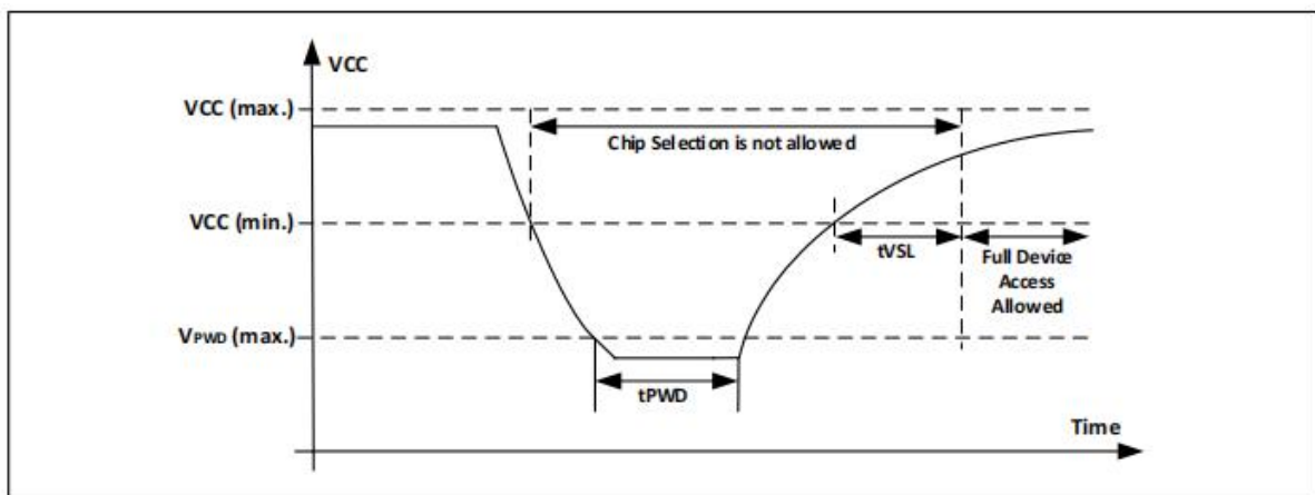
Figure-73. Power-Down and Voltage Drop
