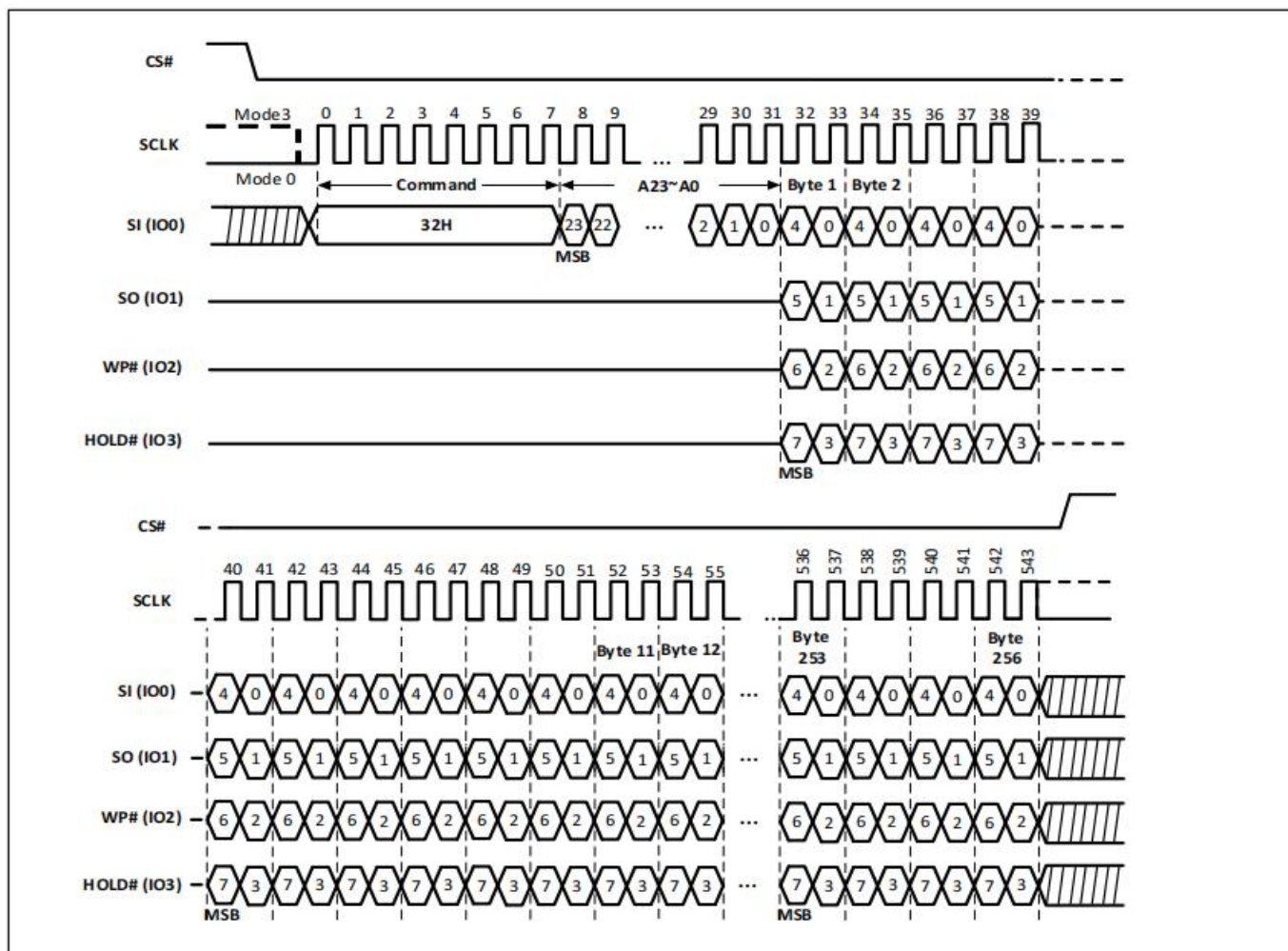
Figure-45. Quad Input Page Program Sequence Diagram
