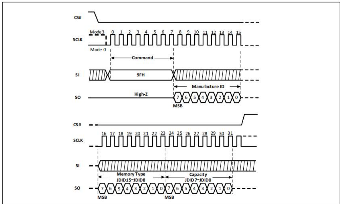
Figure-57. Read Identification Sequence Diagram
