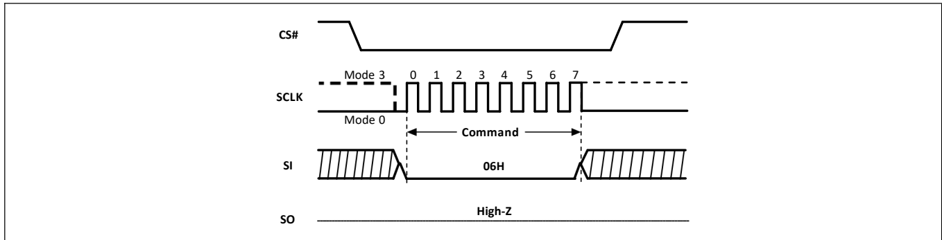
Figure-4. Write Enable Sequence Diagram
