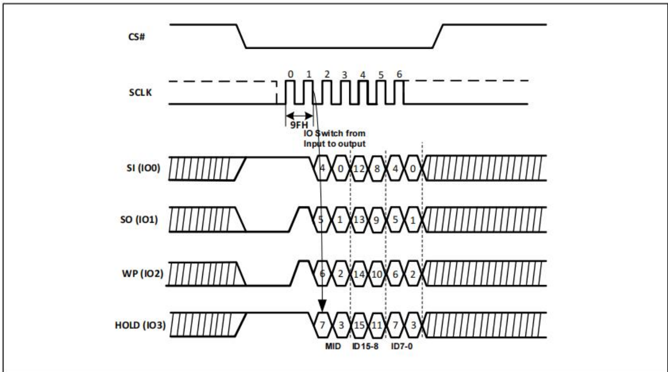
Figure-58. Read Identification Sequence Diagram (QPI)
