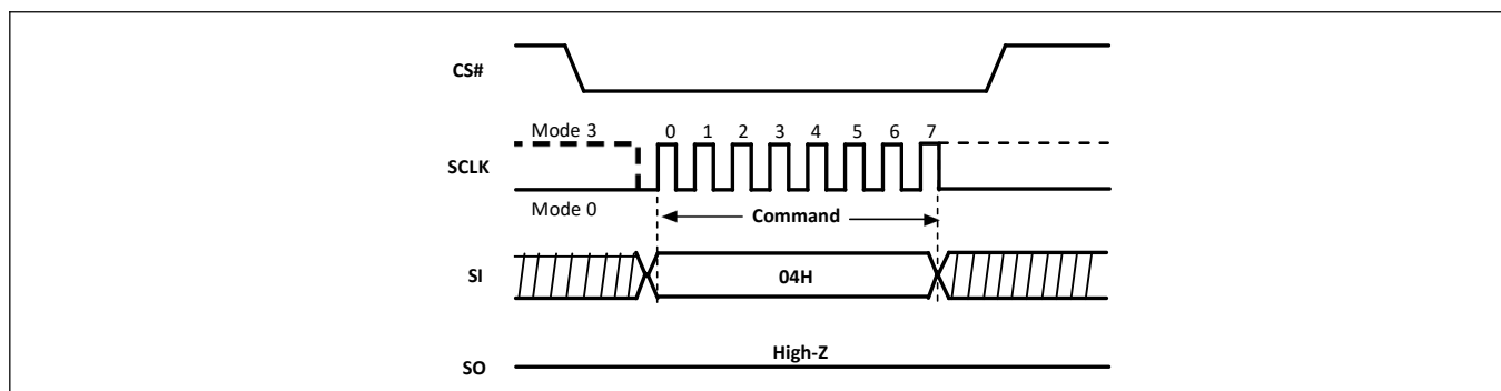
Figure-6. Write Disable Sequence Diagram
