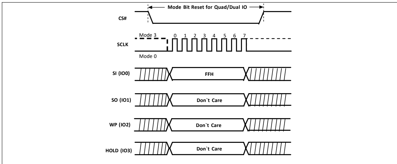
Figure-66. Continuous Read Mode Reset Sequence Diagram
