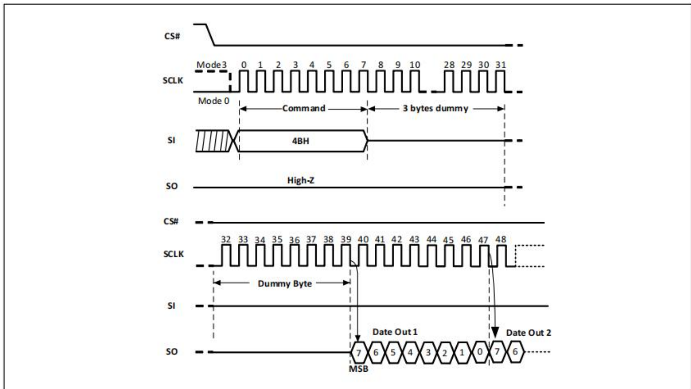
Figure-63. Read Unique ID Sequence Diagram
