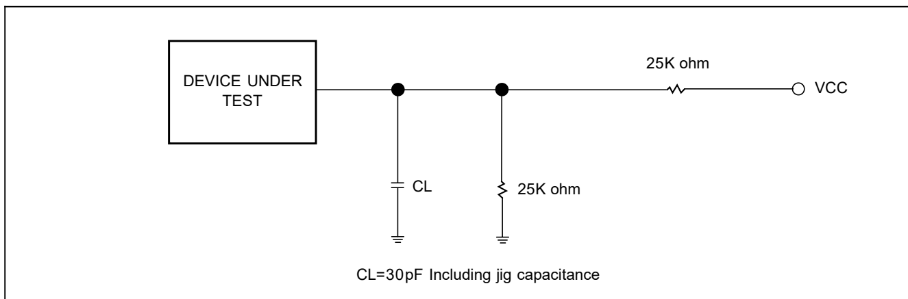
Figure-76. OUTPUT LOADING
