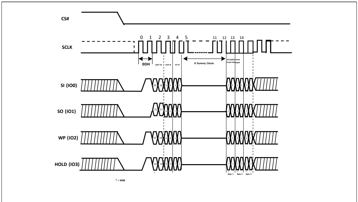
Figure-18. DTR Fast Read Sequence Diagram (QPI)
