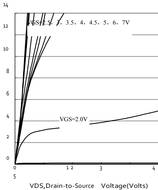
Figure 1. Output Characteristics
