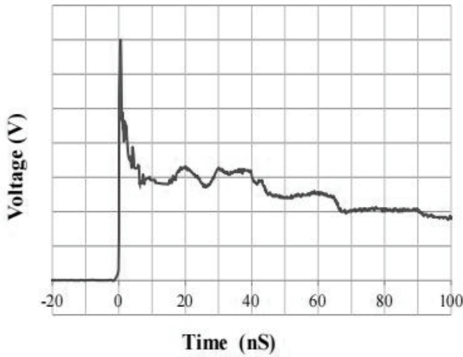
IEC61000-4-2 Pulse Waveform
