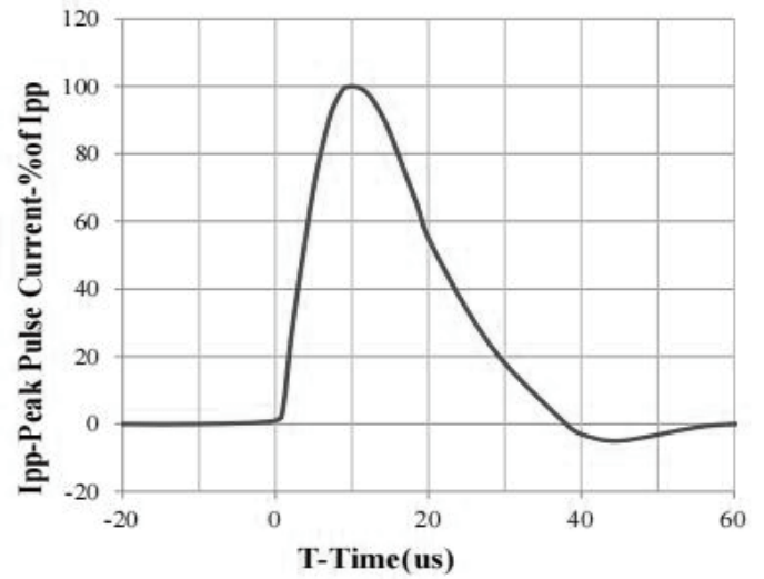
8 X 20us Pulse Waveform
