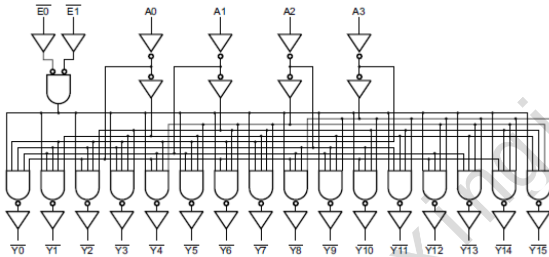
Figure 1. Functional diagram
