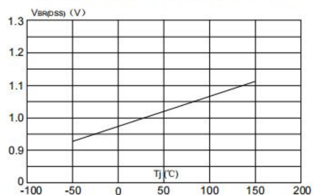
Fig6 Normalized Breakdown Voltage vs. Tj
