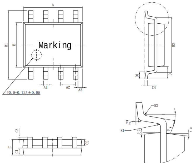
SOP8 Dimension and Mark
