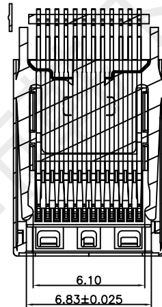
SECTION: B-B SCALE 1:1
