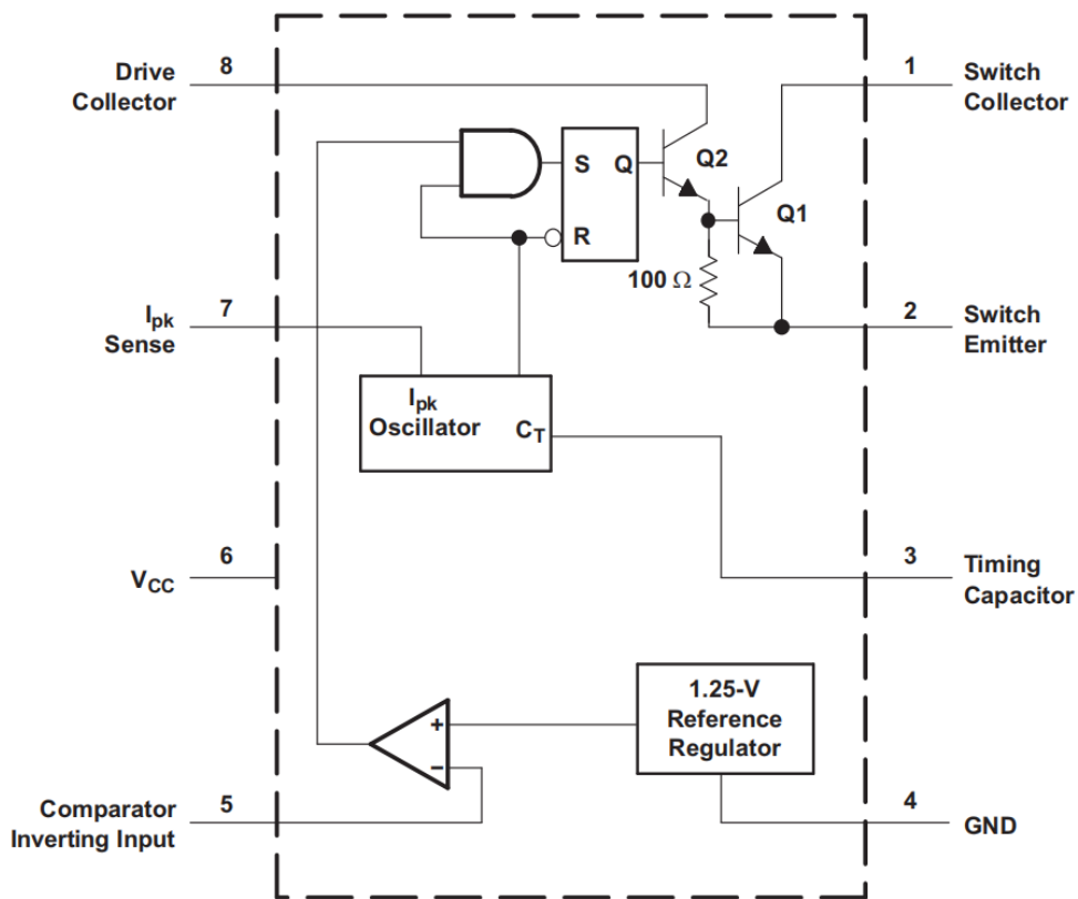
Figure 2.2: MC34063 Functional Block Diagram
