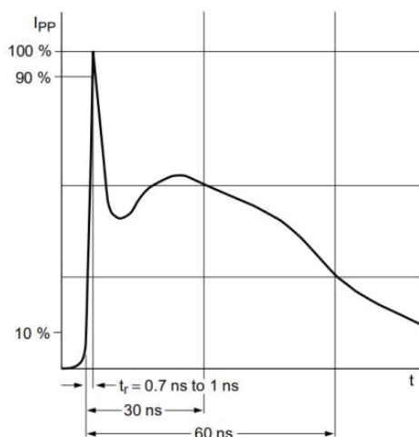
IEC61000-4-2 Waveform
