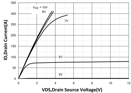
Extended Output Characteristics@T j =25°C
