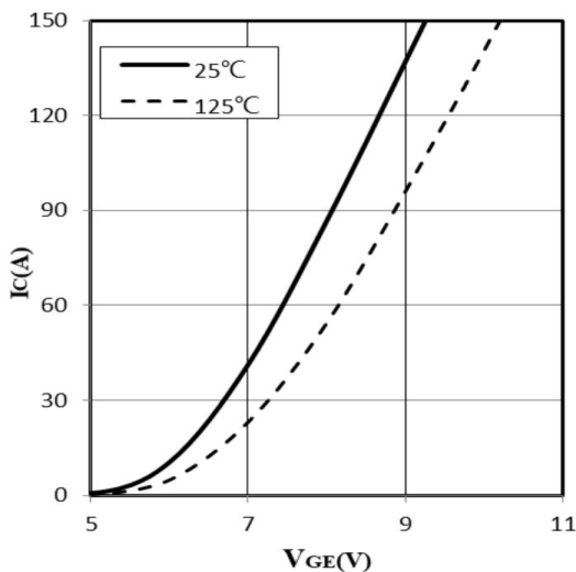
Fig 9. Typical collector-emitter saturation voltage as a function of V_{GE} ( T_j=25^\circ\text{C} )
