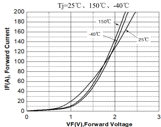
Diode Characteristic
