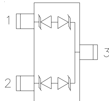
SOT23 (Top View)
