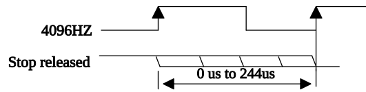
Figure 9. STOP bit release timing
