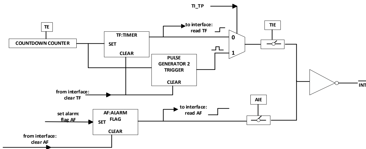
Figure 3. Interrupt scheme
