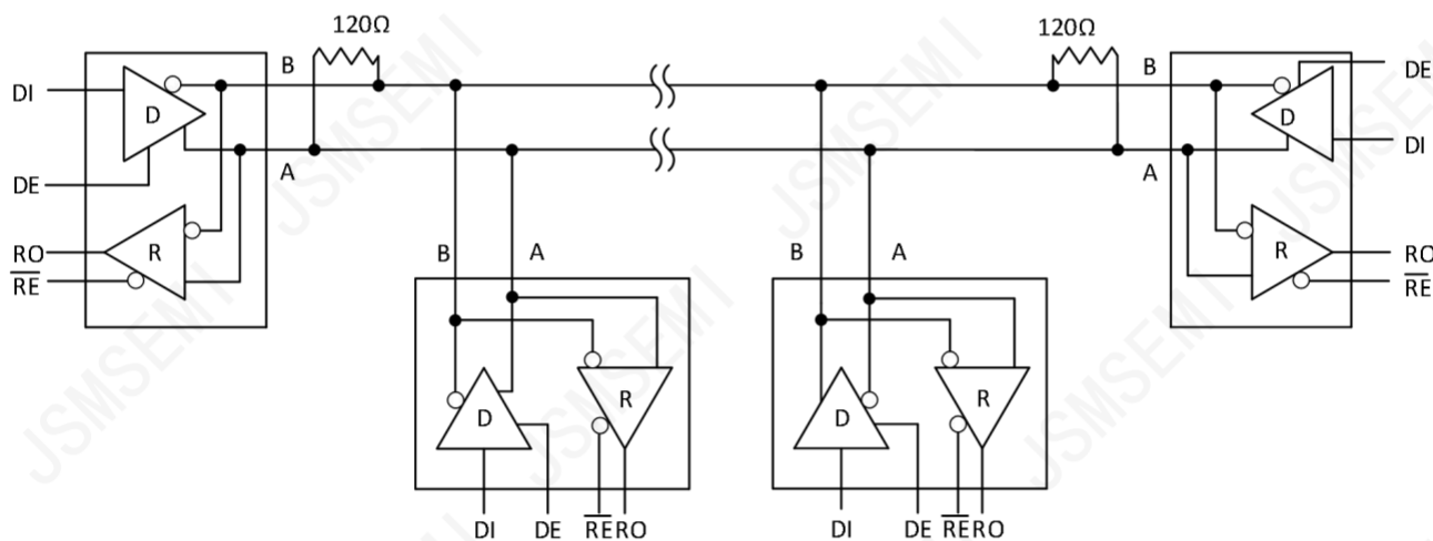
Figure 9. Typical half-duplex RS-485 Network
