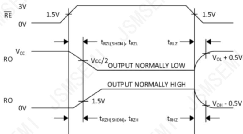
Figure 6. Receiver Enable and Disable Times
