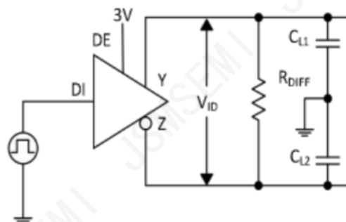
Figure 2. Driver timing test load
