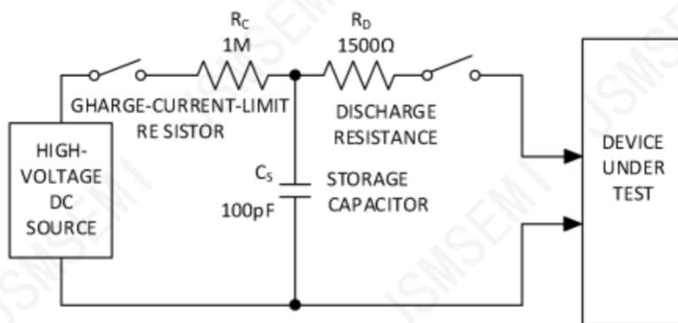
Figure 7a. Human Body ESD Test Model
