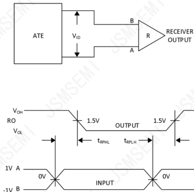
Figure 5. Receiver Propagation Delays
