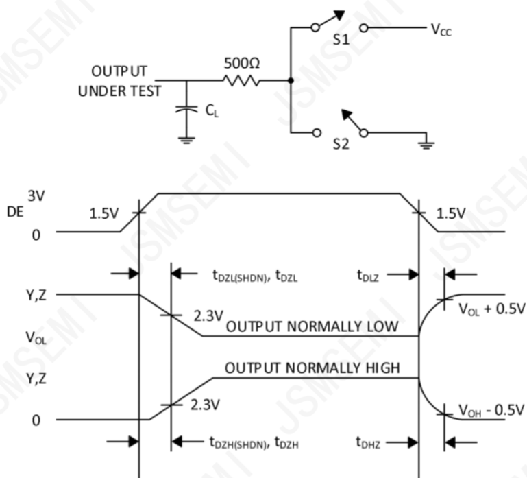
Figure 4. Driver Enable and Disable Times
