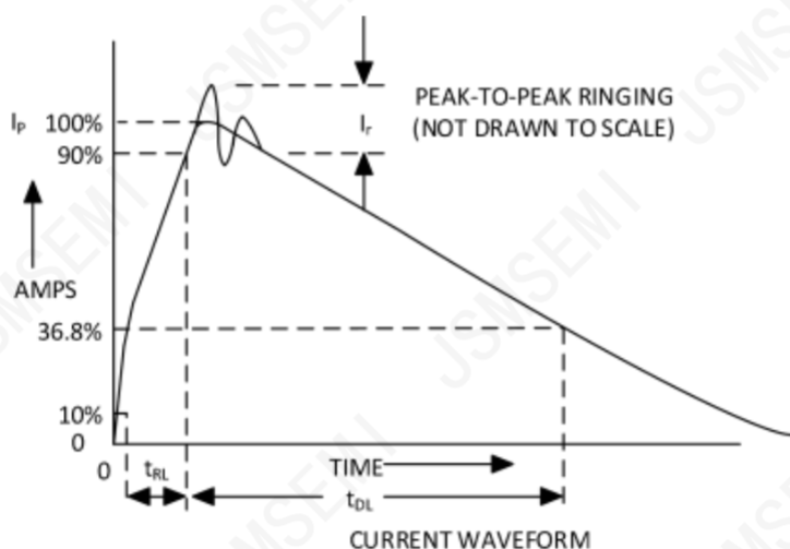
Figure 7b. Human Body Current Waveform
