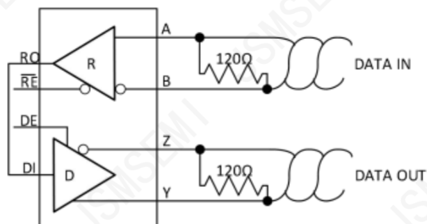
Figure 8. Line repeater for SP485ECN SP485EEN
