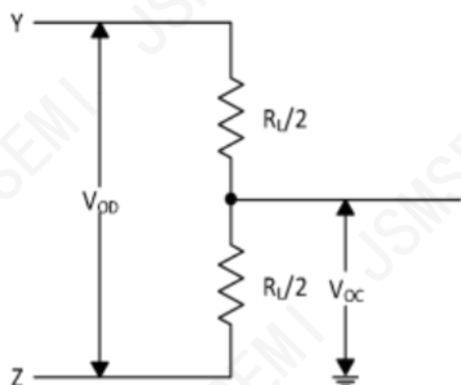
Figure 1. Driver DC Test Load
