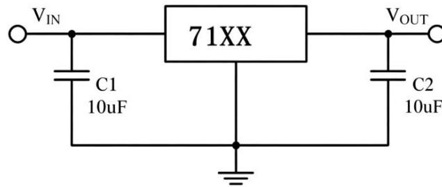
Figure 3. Basic Circuit
