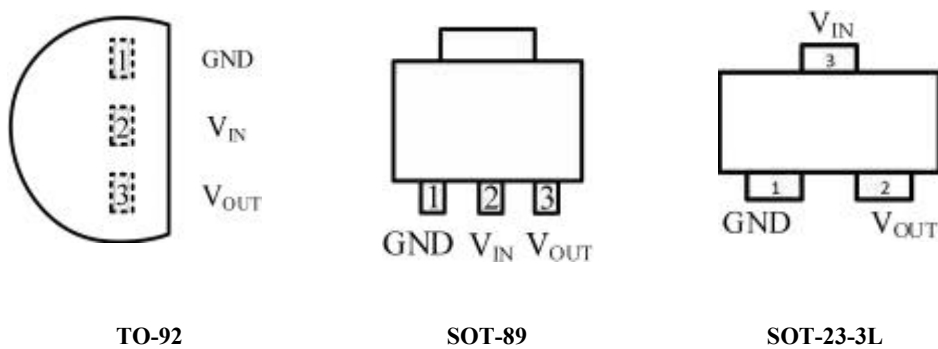
Figure 2.HT75XX Pin
