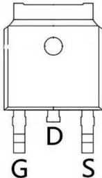
Pin Assignment
