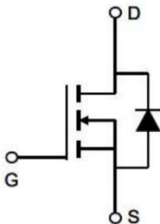
TO252 Pin Configuration
