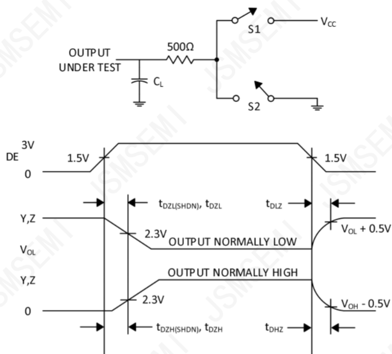
Figure 4. Driver Enable and Disable Times
