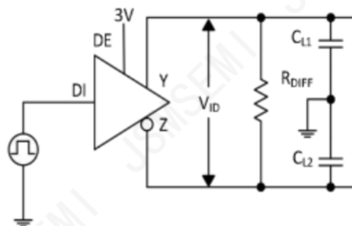
Figure 2. Driver timing test load
