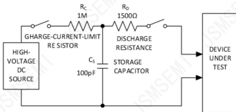
Figure 7a. Human Body ESD Test Model
