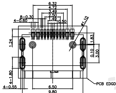
PCB LAYOUT TOLERANCESIZE:±0.05
