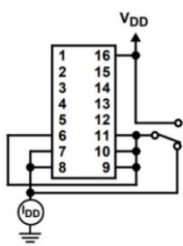
Fig.1 静态电流
