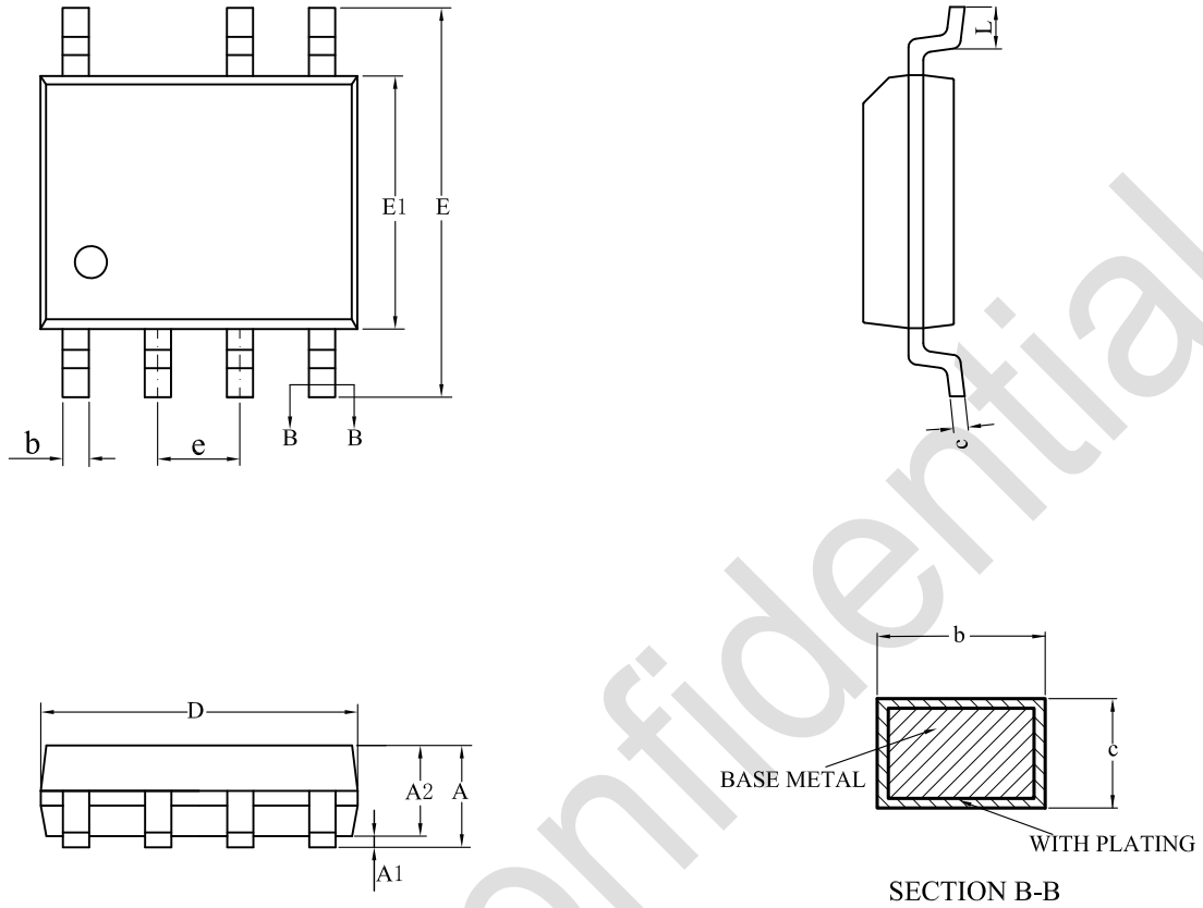
SOP-7 Package Outline Dimensions
