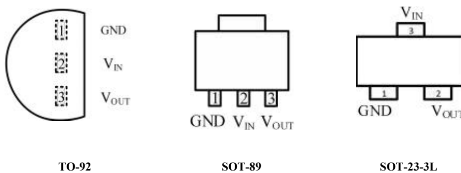
Figure 2.HT75XX Pin
