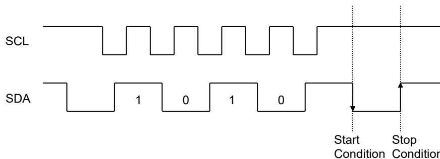
Figure 50. The Case of Cancel by Start, Stop Condition during Target Address Input
