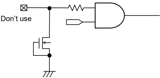
Figure 57. Input Pin Circuit Diagram (A0, A1)
