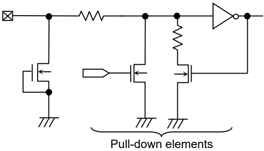
Figure 58. Input Pin Circuit Diagram (A2, WP)
