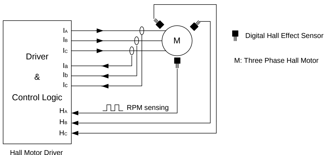
Fig.1 Functional Application Circuit in 3-Phase Hall Motor
