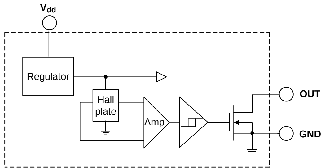
Figure 1. Function Block Diagram of SL1120
