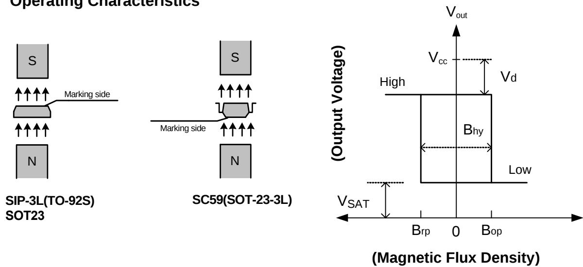
Figure 2. Operating Characteristics of SL1120
