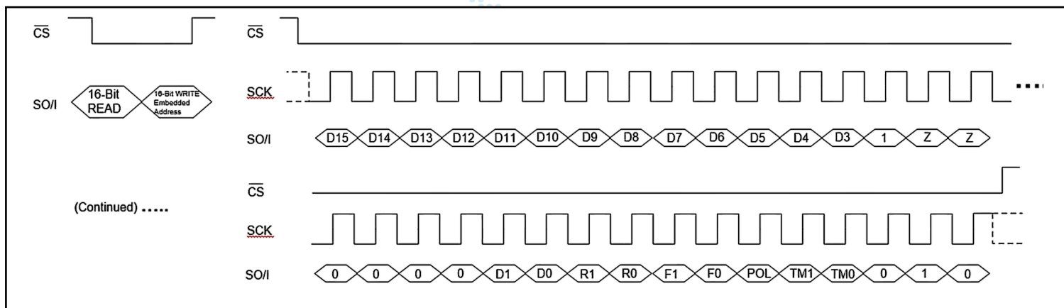
Figure 4. Read and write control registers
