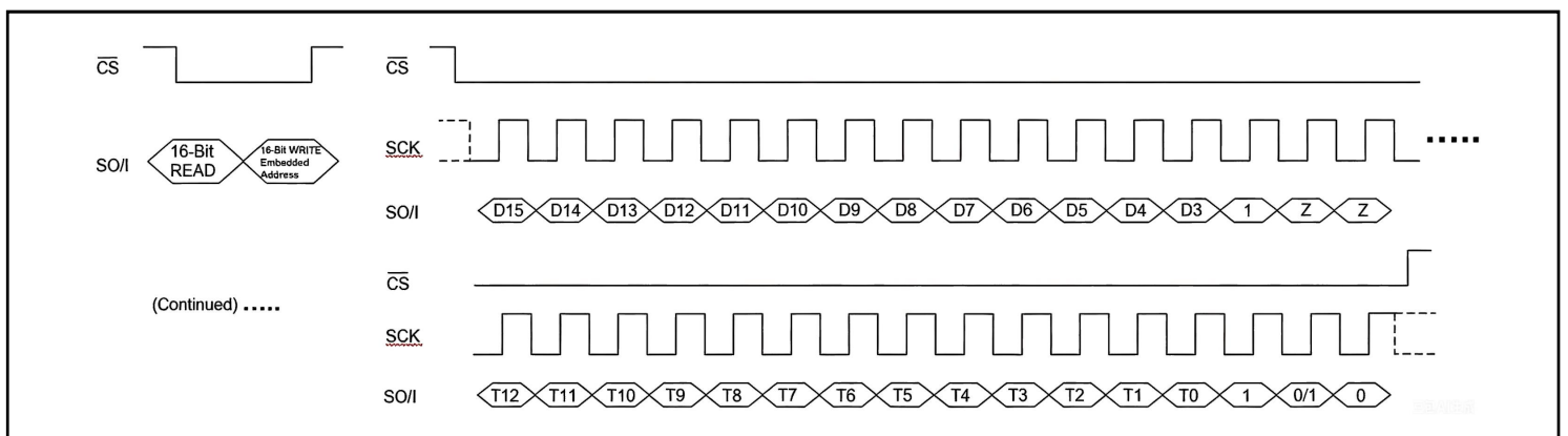
Figure2. Multiple Command Sequence
