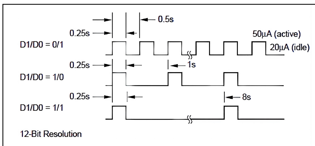
Figure 9. Interpretation of Conversion Time and Period
