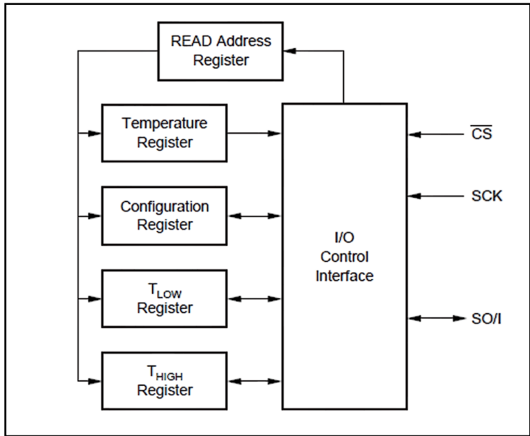
Figure 7. Internal register structure of .TMP122
