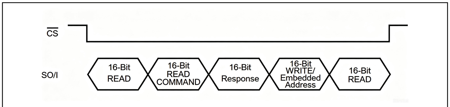
Figure2. Multiple Command Sequence
