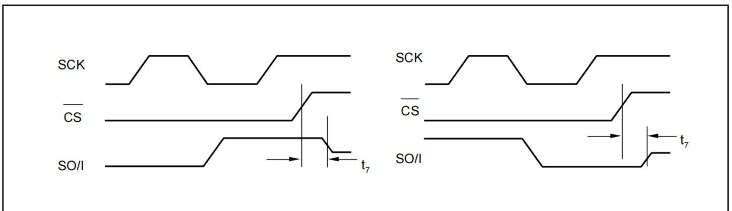
Figure 11. High-impedance output timing diagram
