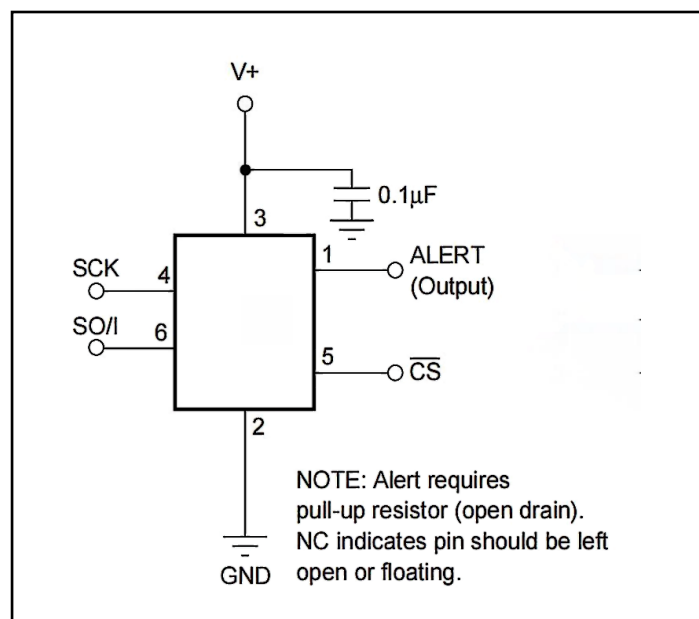
Figure 1. Typical connection of TMP122
