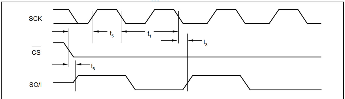
Figure 10. Output data timing diagram.
