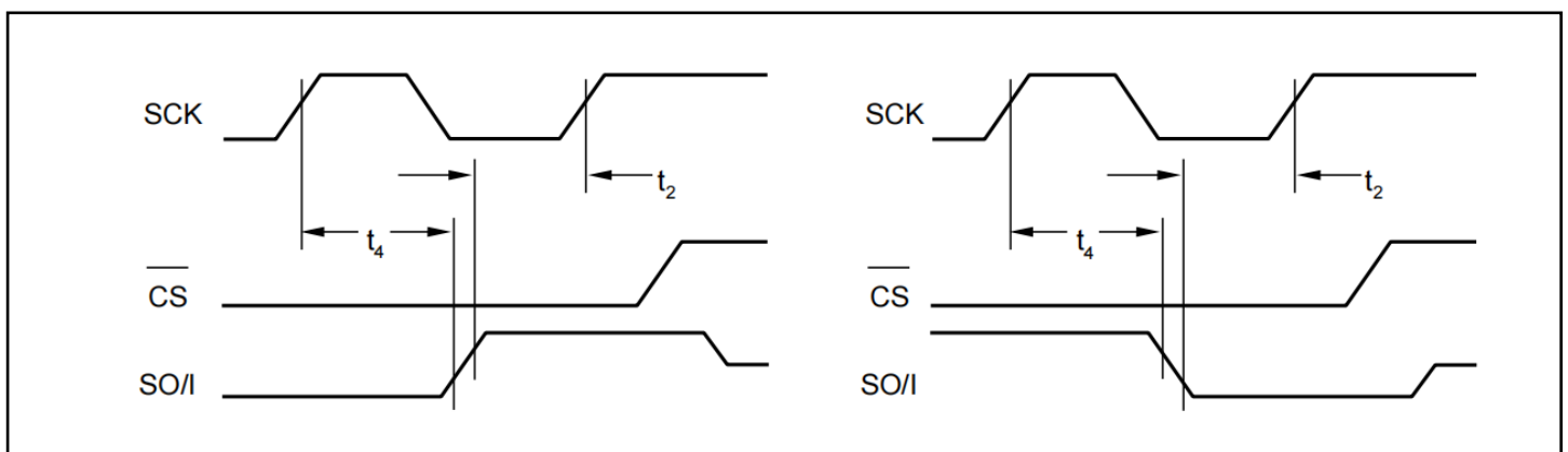
Figure 12. Input Data Timing Diagram
