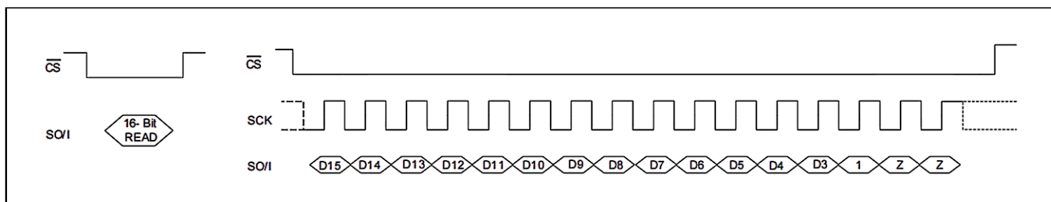
Figure 6. Read data
