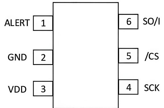
PIN CONFIGURATIONS
