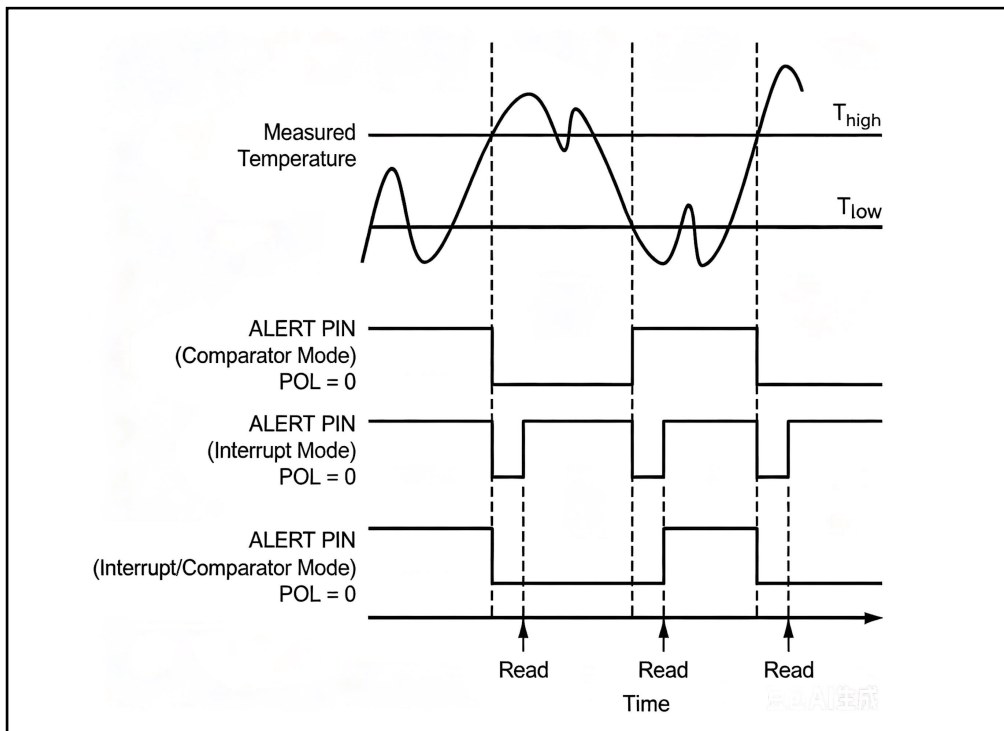
Figure 8. ALERT Output Transfer Equation
