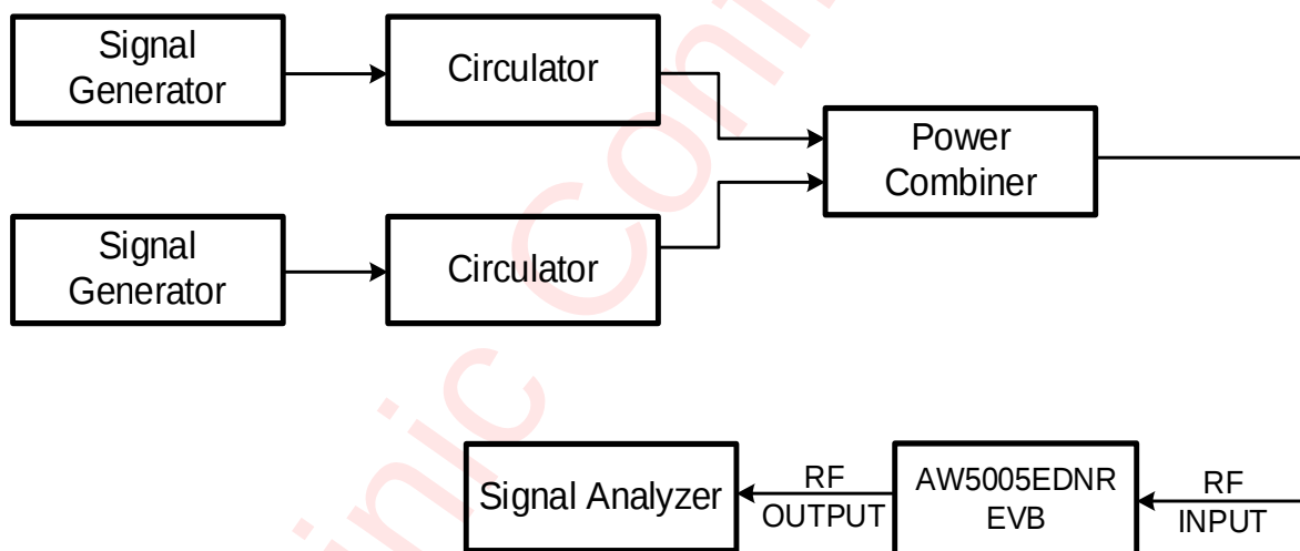
Figure 7 Intermodulation Distortion Test
