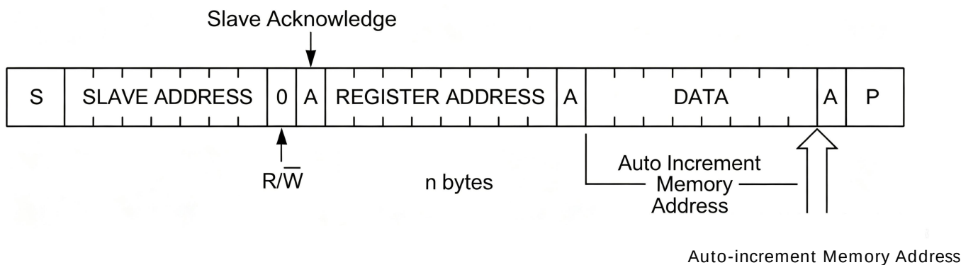
Figure 11 Main Transmitter to Slave Receiver (write Mode)
