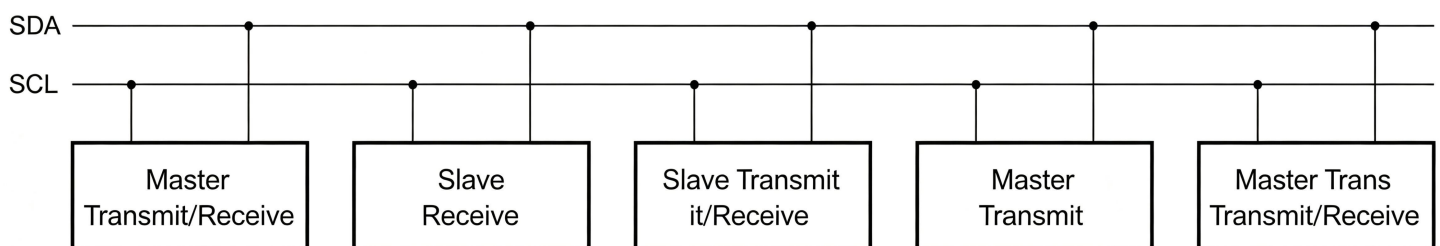
Figure 6 Configuration Diagram of the I 2 C Bus System
