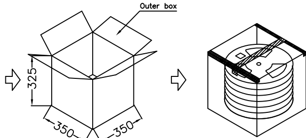
Outer box
