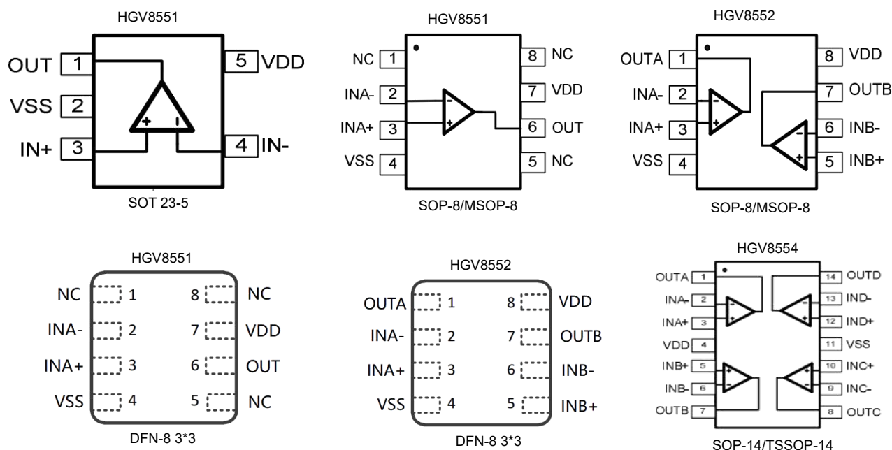
Figure 1. Pin Assignment Diagram
