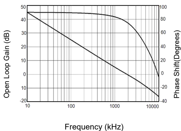
Open Loop Gain, Phase Shift vs. Frequency at +2.5V
