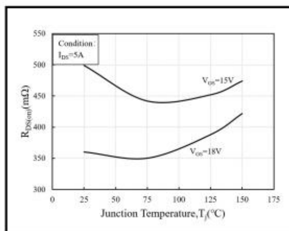
Fig.12 On-Resistance vs Temperature For Various Gate
