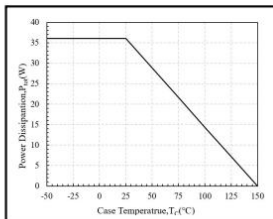
Fig. 14 Maximum Power Dissipation Derating vs Case Temperature
