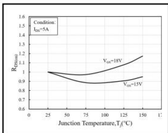
Fig.11 Normalized On-Resistance vs Temperature
