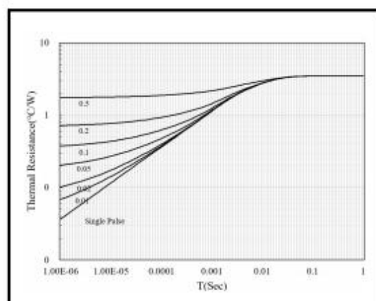
Fig. 16 Transient Thermal Impedance (Junction-Case)
