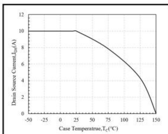
Fig. 15 Continuous Drain Current Derating vs Case Temperature
