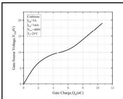
Fig.19 Gate Charge Characteristics
