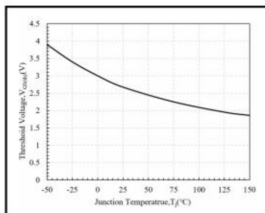
Fig. 18 Threshold Voltage vs Temperature
