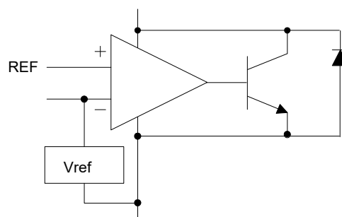
Figure 2. Functional Block Diagram of TL431
