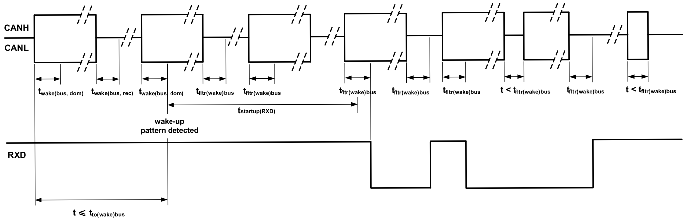
Figure 7-2 Wake-Up Timing
