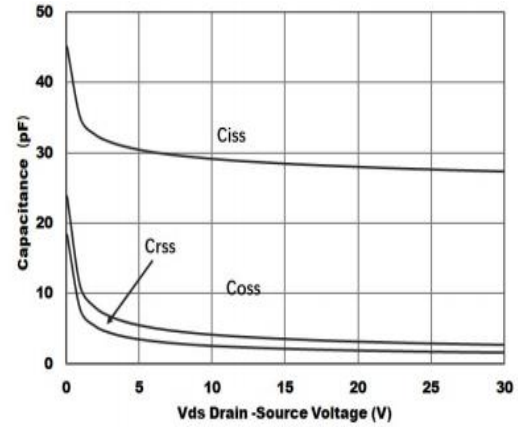
Figure 4: Capacitance Characteristics
