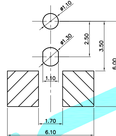
PCB WELDING DIMENSIONS
