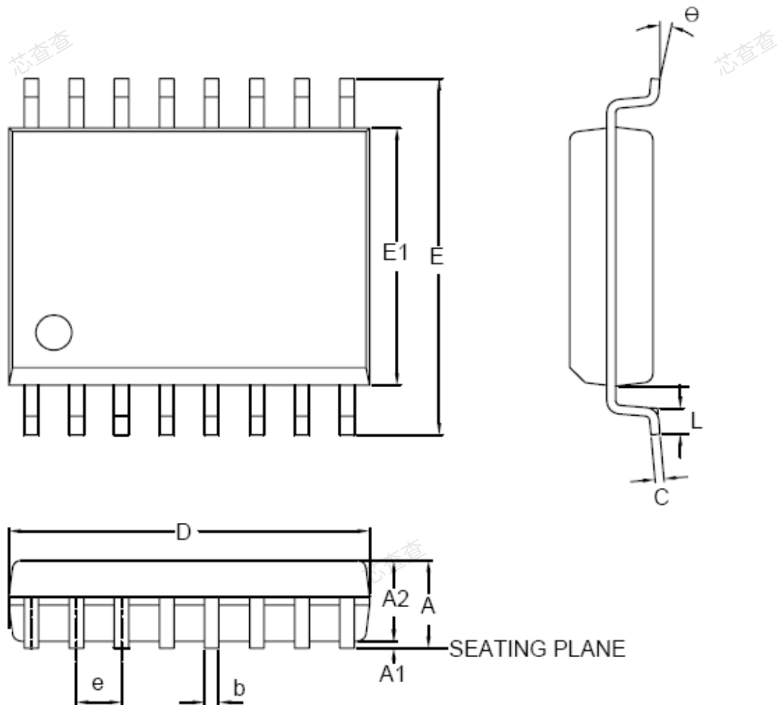
Figure 35. 16 LEAD SOP 300 mil
