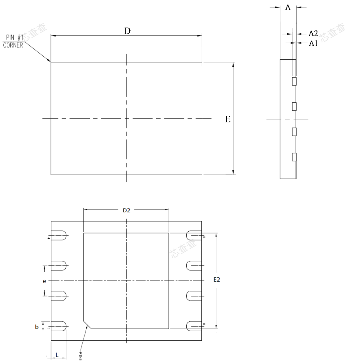
Figure 36. VDFN 8 ( 5x6 mm )
