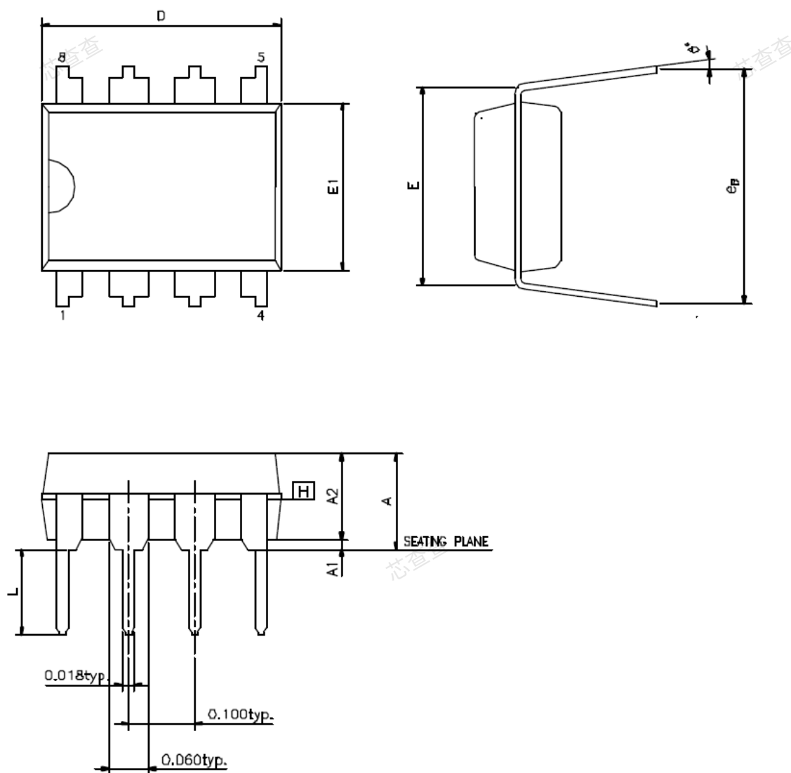
Figure 37. PDIP8
