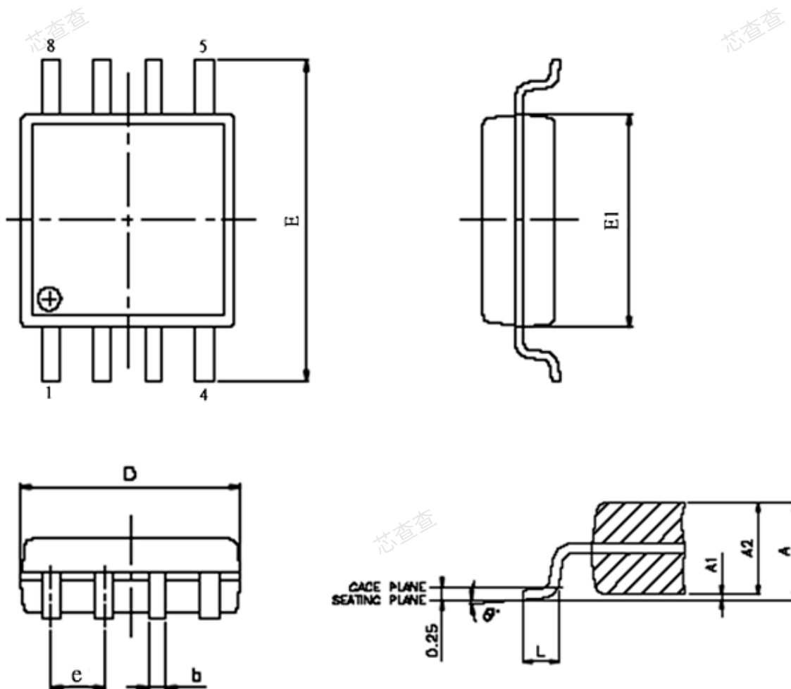
Figure 34. SOP 200 mil ( official name = 208 mil )
