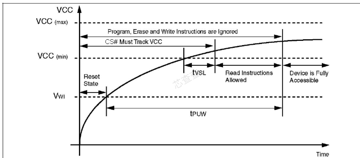
Figure 30. Power-up Timing
