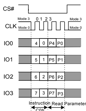
Figure 7.38 Set Read Parameters Instruction (QPI Mode only)
