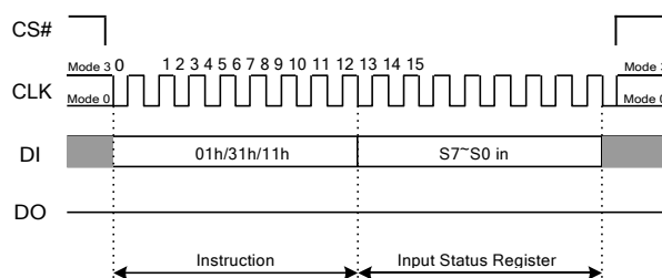
Figure 7.5a Write Status Register Instruction(SPI Mode)
