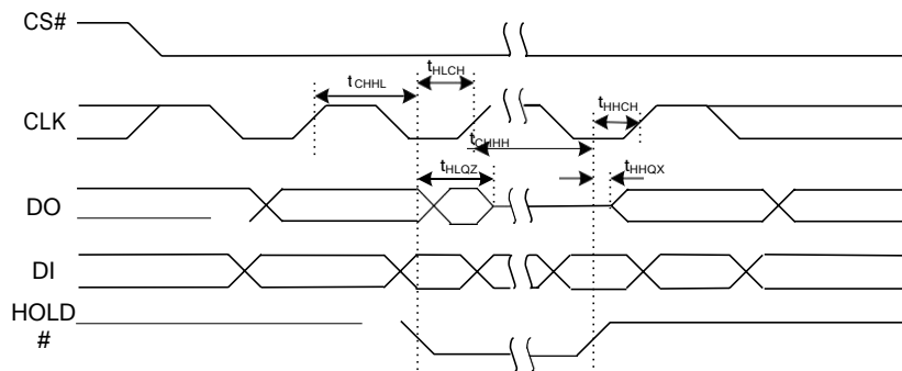
Figure 8.6 Hold Timing
