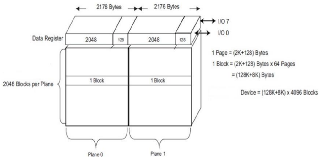
Figure 6. Array Organization
