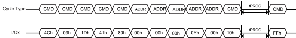
Figure 16. Timing Diagram for the PBP Sequence
