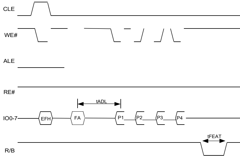
Figure 9. Set Features Timing [18, 19, 20]
