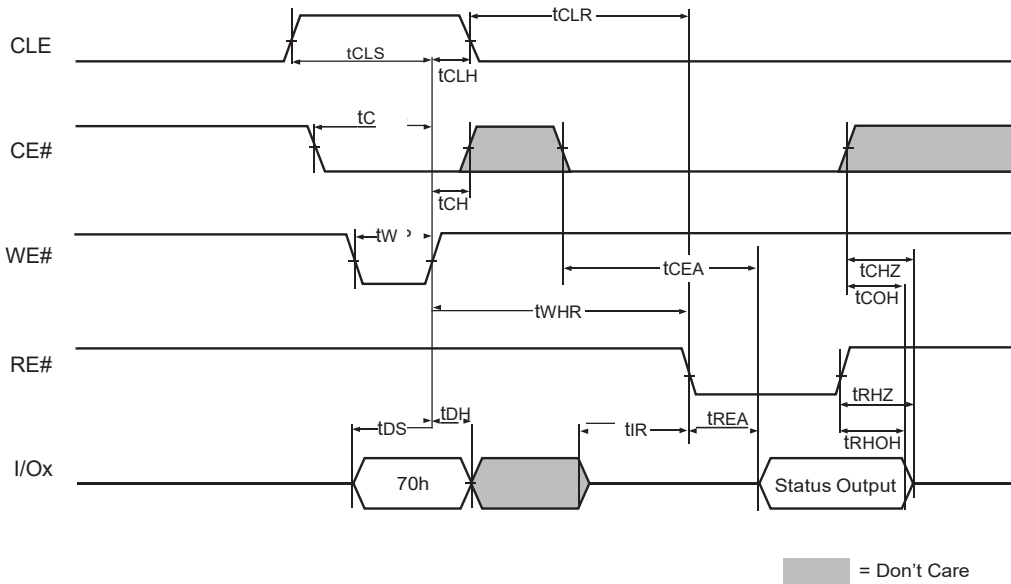
Figure 44. Read Status Cycle
